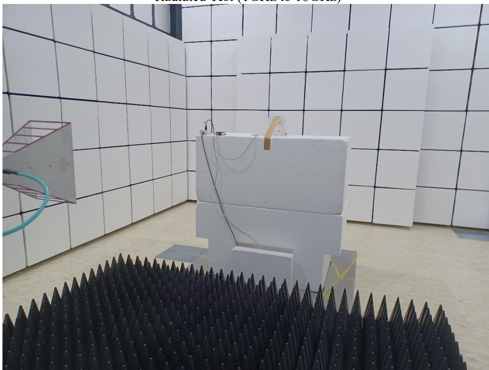
Radiated Test (1GHz to 18GHz)
