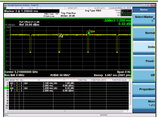
802.11ac-VHT80 (T = 1.145ms)
