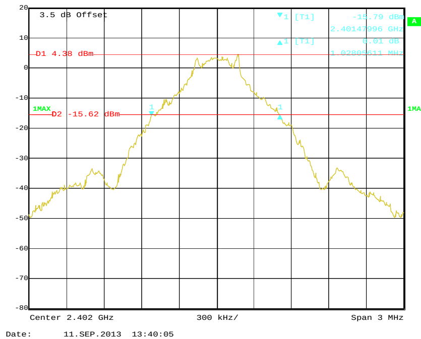
a 1 [T1] RBW 30 kHz RF Att 30 dB 0.01 dB VBW 100 kHz 1.02805611 MHz SWT 8.5 ms Unit dBm
