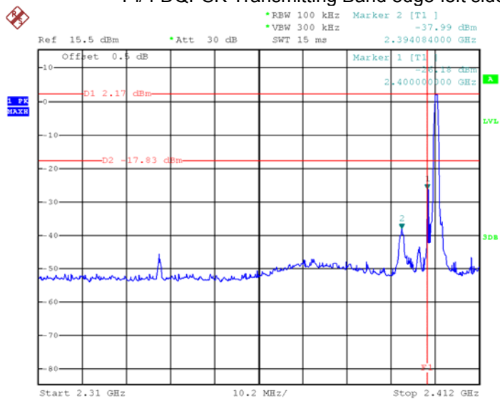
Pi/4 DQPSK Transmitting Band edge-left side
