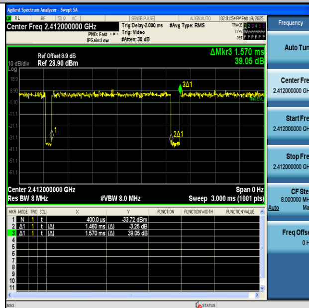
NTNV-11AX20SISO-Ant1-2412
