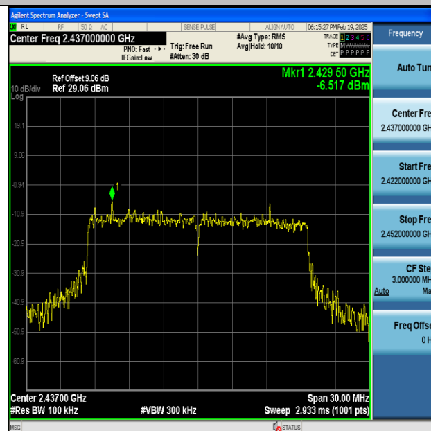
11AX20SISO-Ant1-2437-0~Reference-PASS
