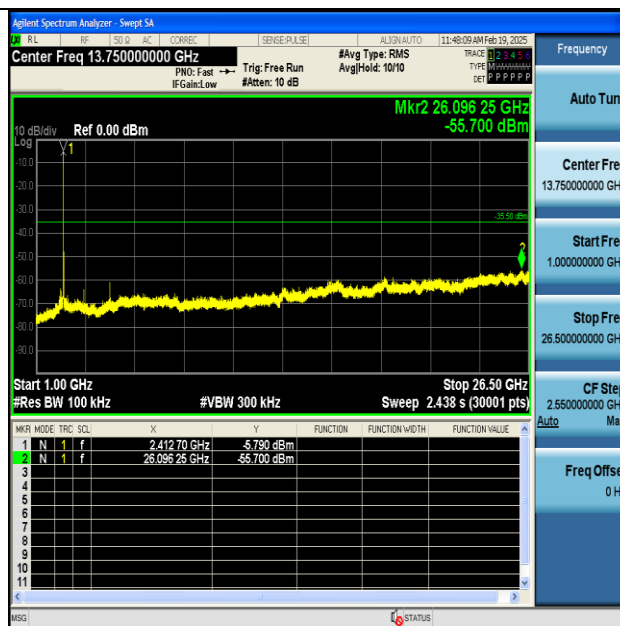
11B-Ant1-2412-1000~26500-PASS
