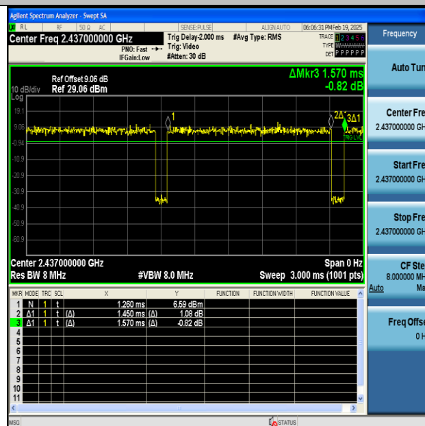
NTNV-11AX20SISO-Ant1-2437
