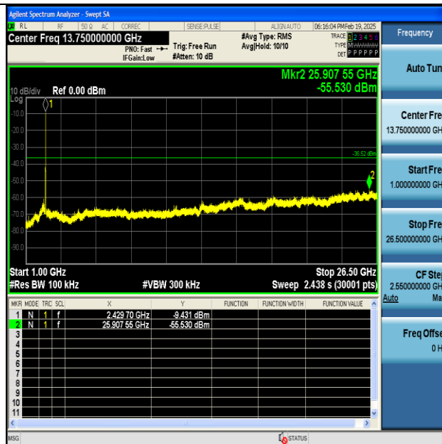
11AX20SISO-Ant1-2437-1000~26500-PASS
