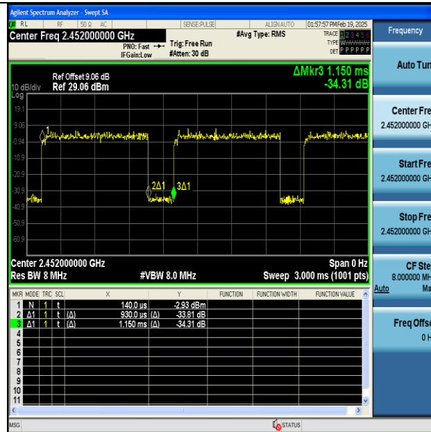
NTNV-11N40SISO-Ant1-2452
