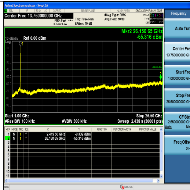
11AX20SISO-Ant1-2412-1000~26500-PASS
