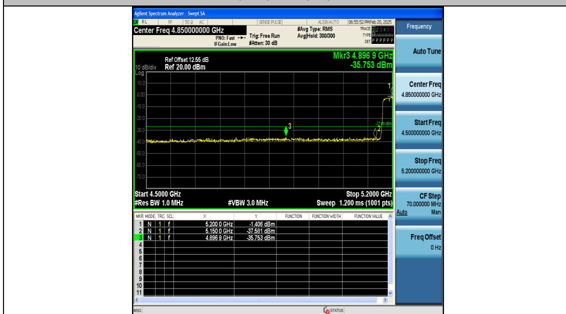
11N40SISO-Ant1-5190-PASS
