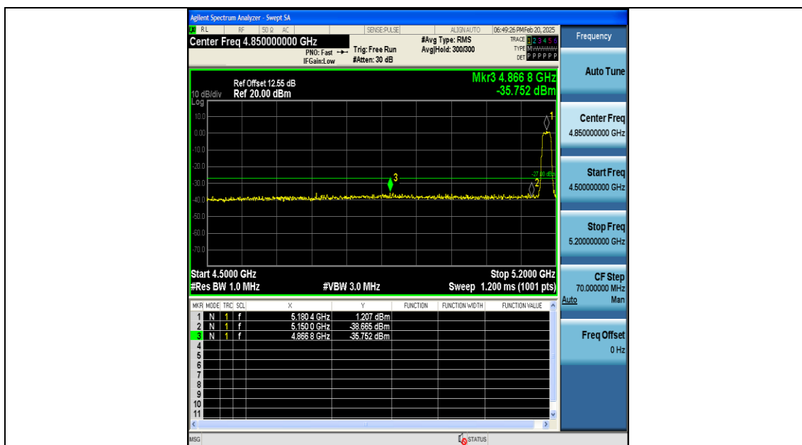
11N20SISO-Ant1-5180-PASS
