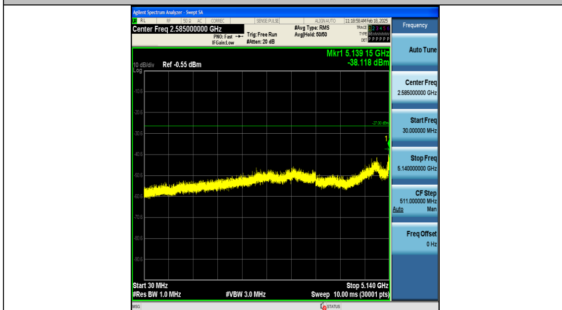
11AC40SISO-Ant1-5190-30~5140-PASS
