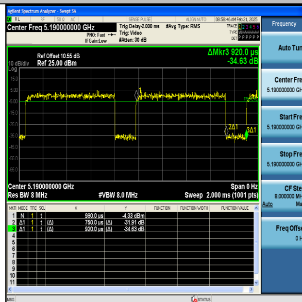
NTNV-11AX40SISO-Ant1-5190
