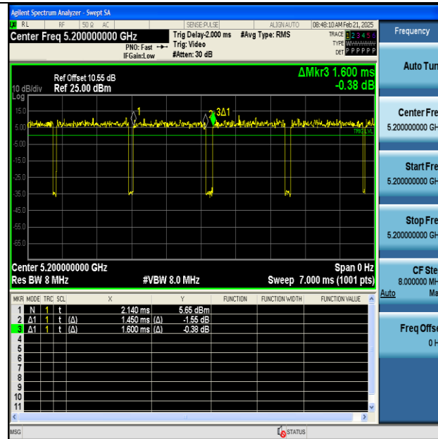
NTNV-11AX20SISO-Ant1-5200
