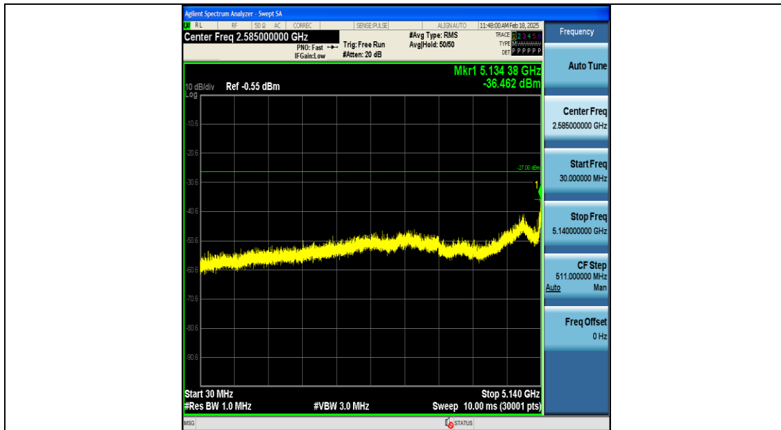
11AX40SISO-Ant1-5190-30~5140-PASS
