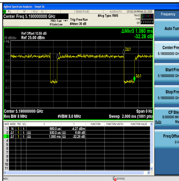
NTNV-11AC40SISO-Ant1-5190
