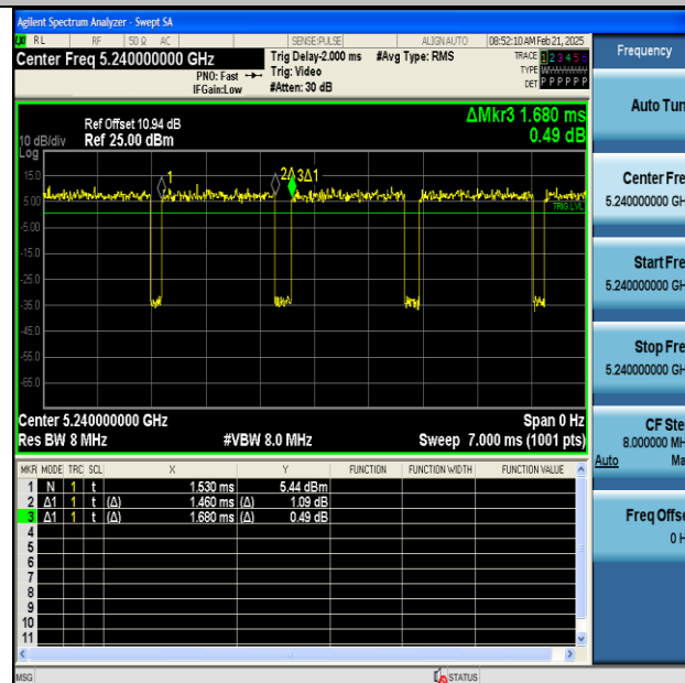
NTNV-11AX20SISO-Ant1-5240
