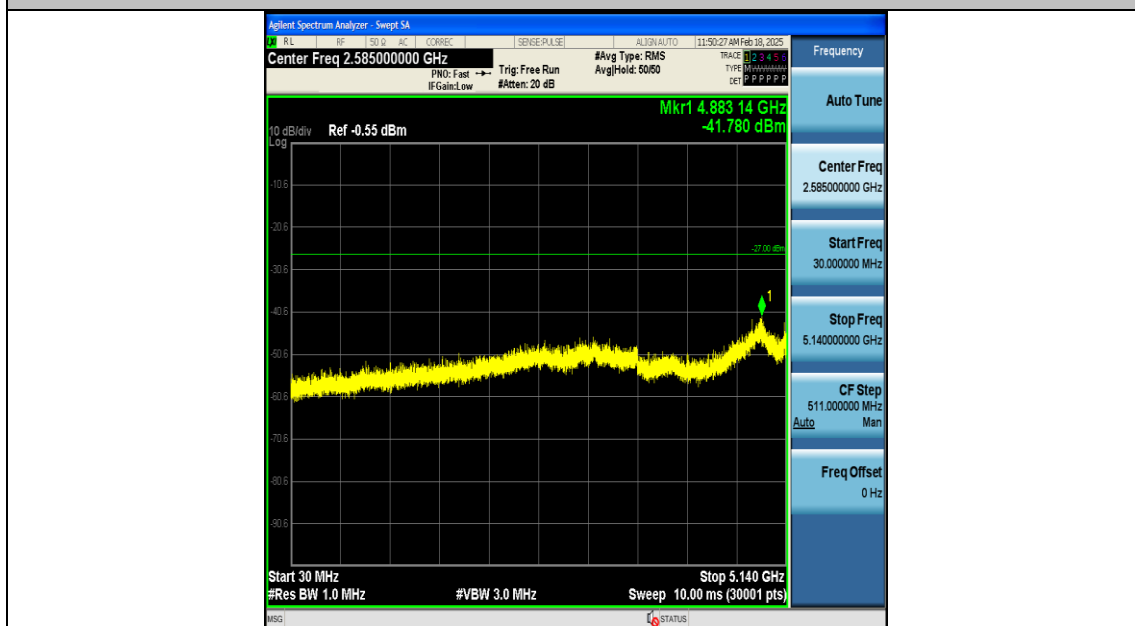
11AX40SISO-Ant1-5230-30~5140-PASS
