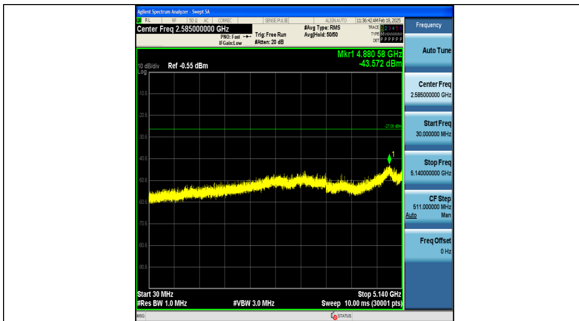
11AX20SISO-Ant1-5180-30~5140-PASS
