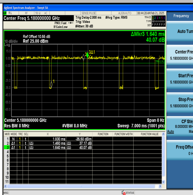
NTNV-11AX20SISO-Ant1-5180
