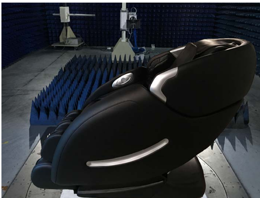
Photograph of set-up for Radiated Emission above 1GHz
