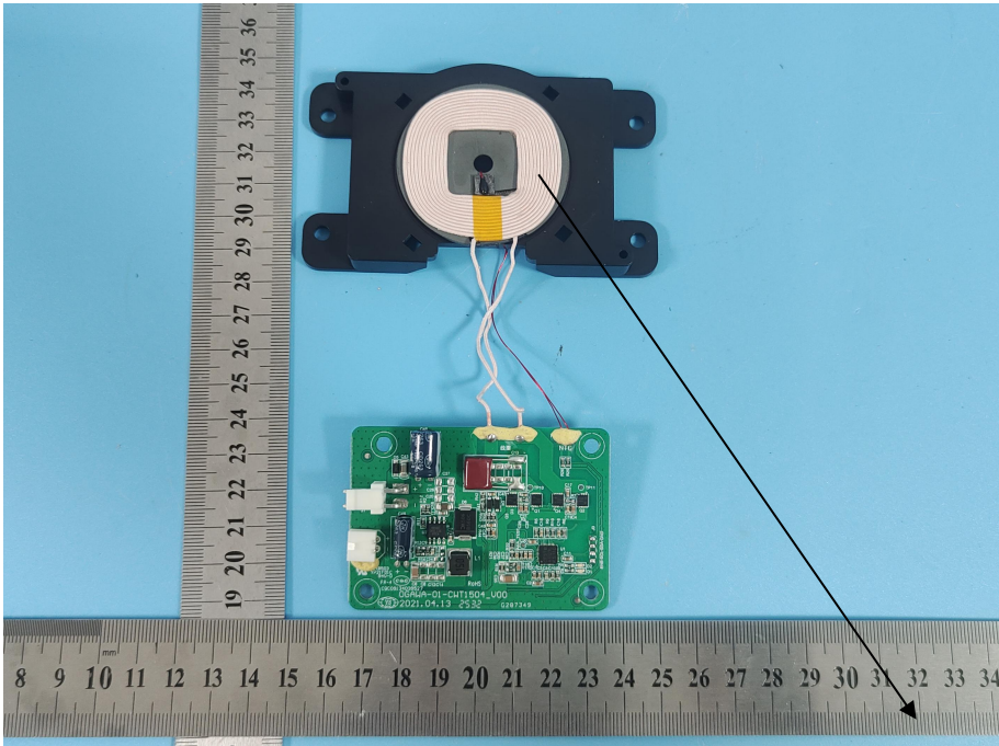
Antenna location
