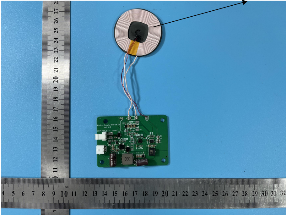
Antenna location
