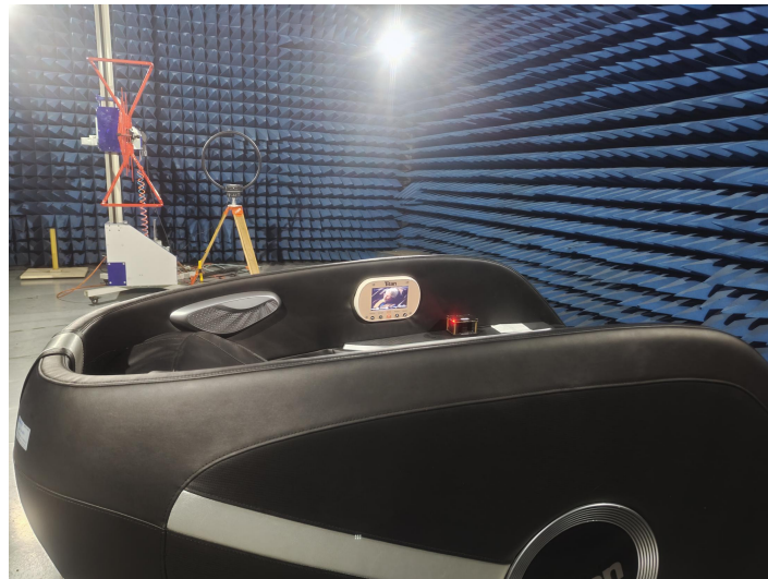
Radiated emission ( 9k-30M )
