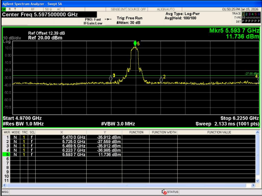
Out Of Band Emission IEEE 802.11n_Channel 118_40MHz_Antenna 0
