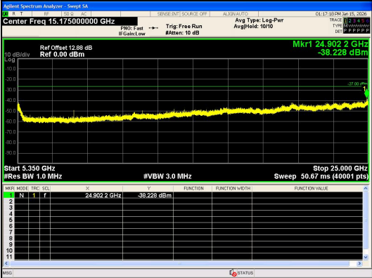
Spurious Emission:5350~25000.0 MHz IEEE 802.11n_Channel 62_40MHz_Antenna 0
