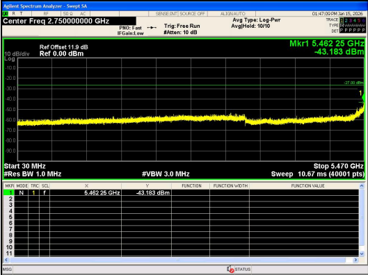
Spurious Emission:30.0~5470 MHz IEEE 802.11n_Channel 102_40MHz_Antenna 0
