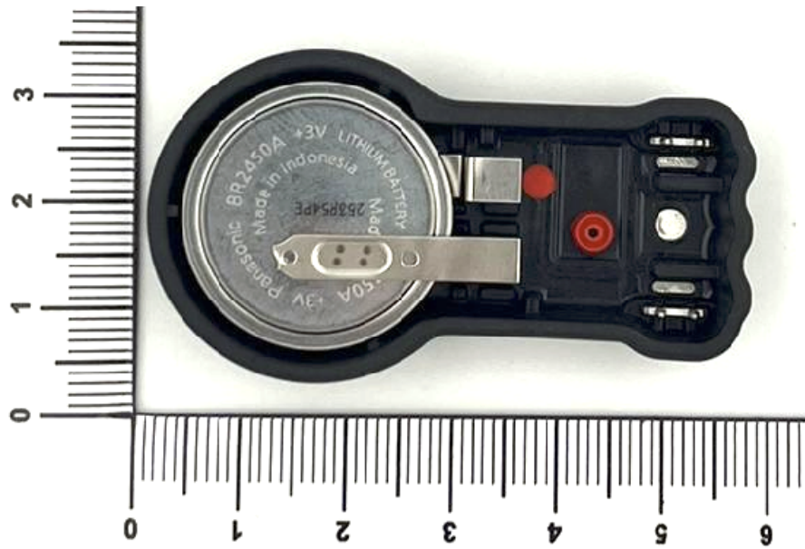
Battery assembled in housing
