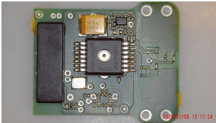
Electronic top side
