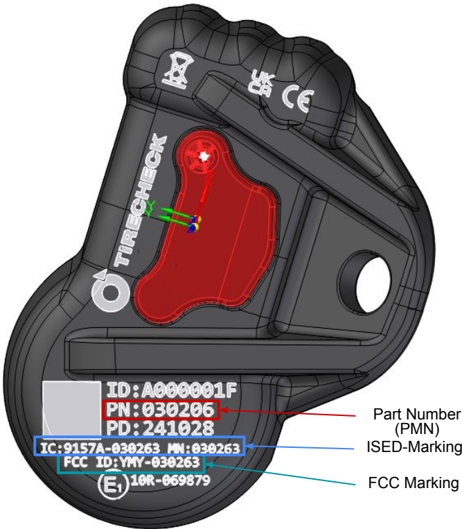
Part Number 030206
