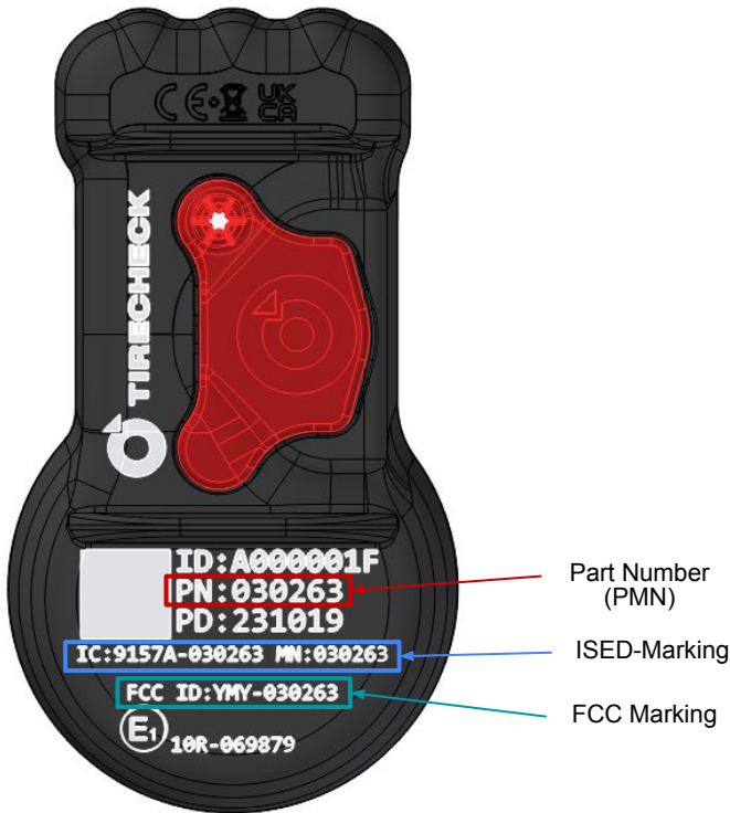
Part Number 030263
