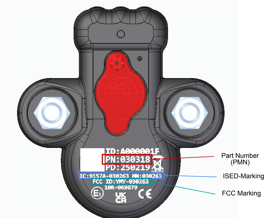
Part Number 030318
