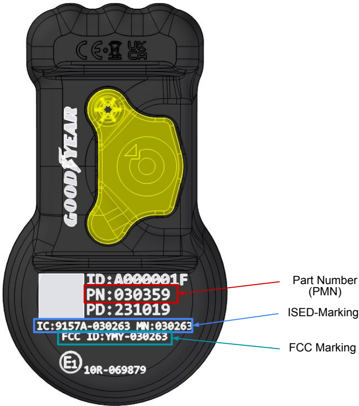
Part Number 030359
