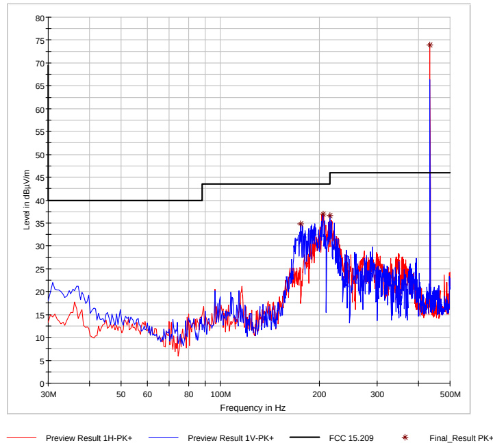
Prescan 30 MHz – 500 MHz
