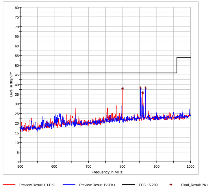
Prescan 500 MHz – 1 GHz
