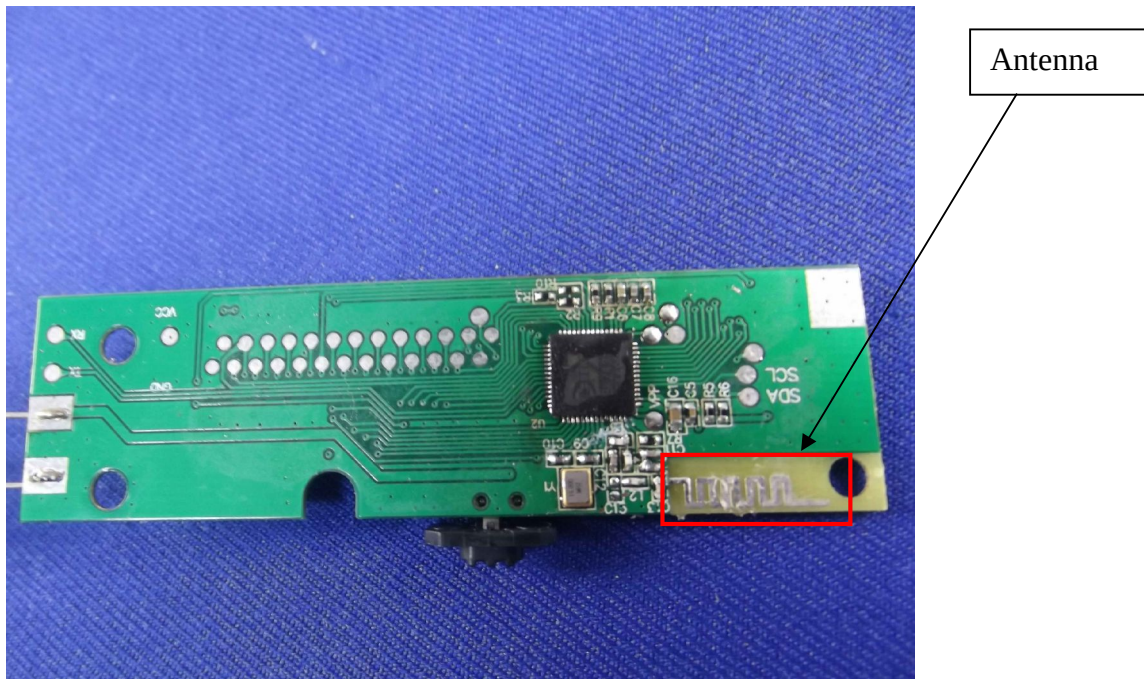
Figure 10 PCB of the EUT-Module View
