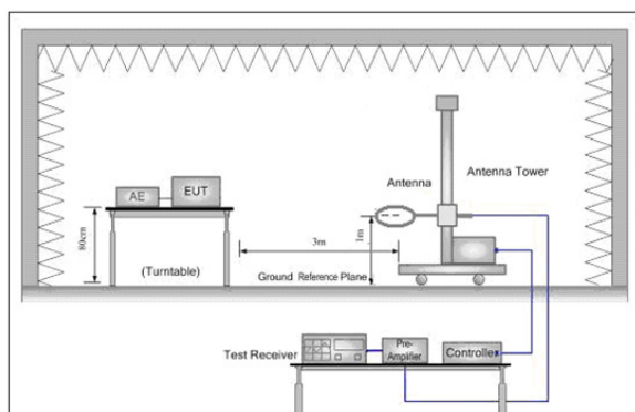
Figure 1. Below 30MHz
