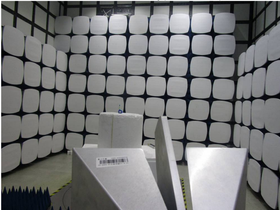
Radiated Emissions Test Setup(abvove 1GHz)
