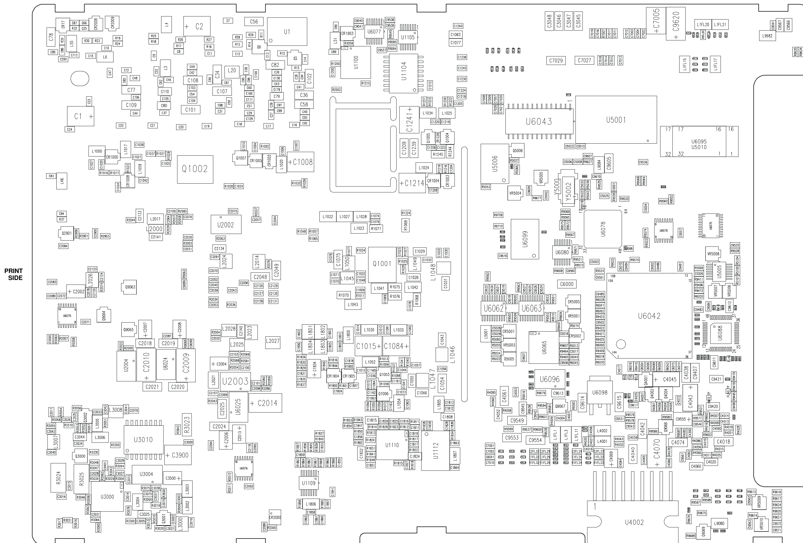
Figure B-3.B. LORD Module, Identification of Components (Sheet 2 of 2)
