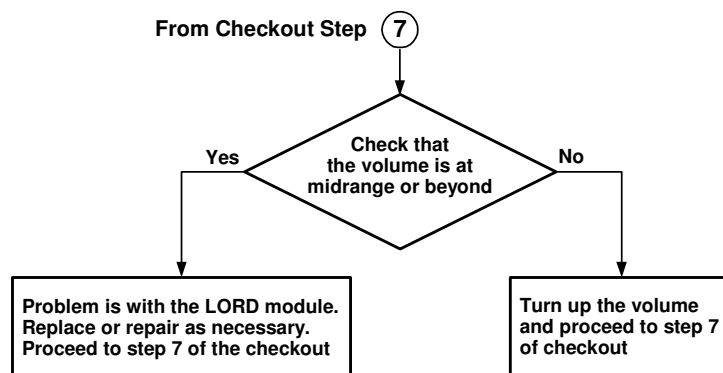
Figure 3-7. MICOM-Z Troubleshooting Chart 6
