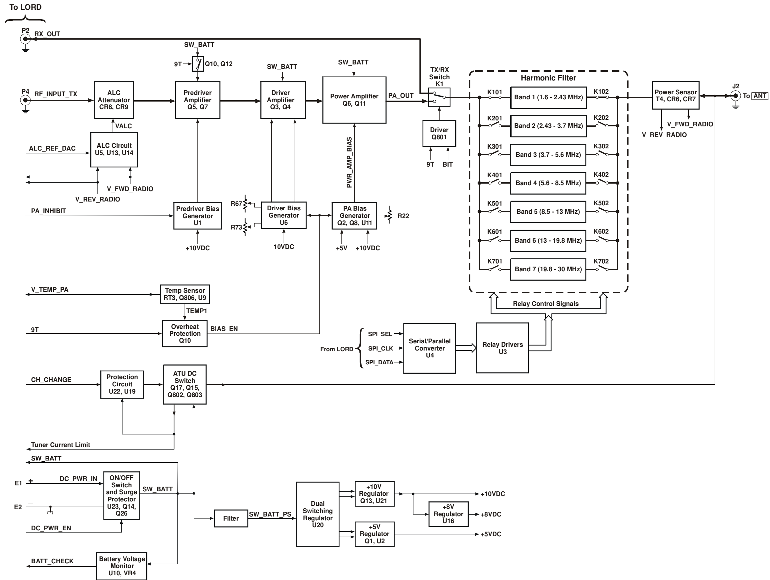
Figure 2-17. HI POWER Module, Functional Block Diagram
