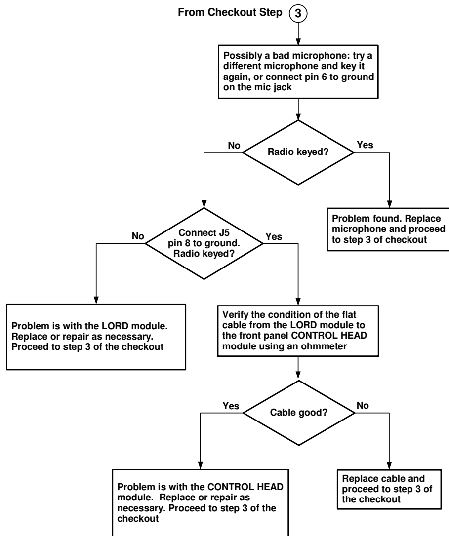
Figure 3-4. MICOM-Z Troubleshooting Chart 3
