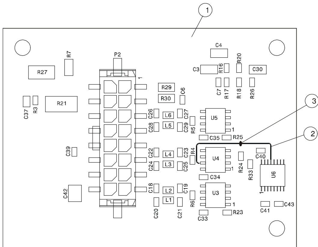
COMPONENT SIDE
