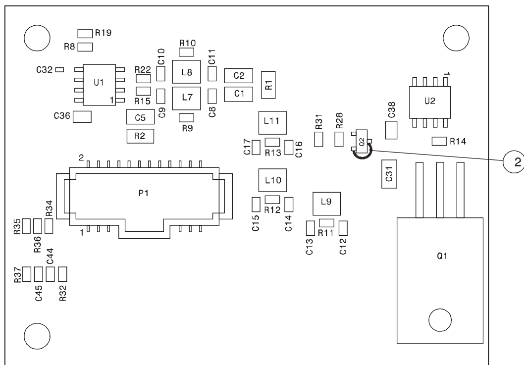
PRINT SIDE
