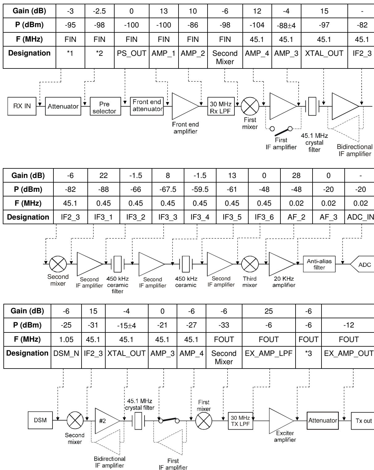
Figure 2-15. LORD Module, Typical Test Point Signal Frequencies and Levels
