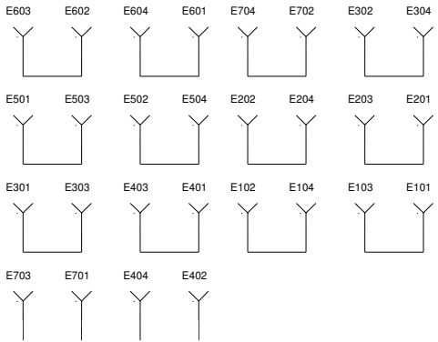
Figure A-2.D. HI POWER Module, Schematic Circuit Diagram (Sheet 4 of 6 – Harmonic Filter, Part II)
