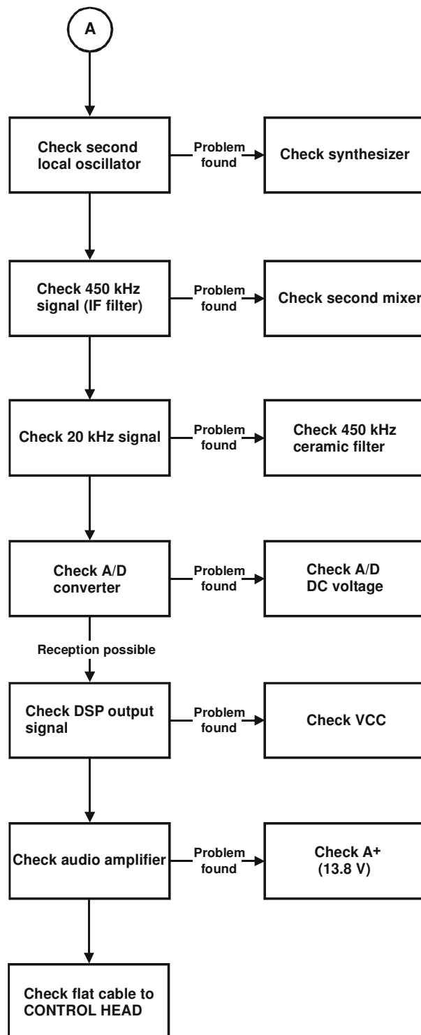
Figure 3-9.B. Receiver Troubleshooting Flowchart (Sheet 2 of 2)
