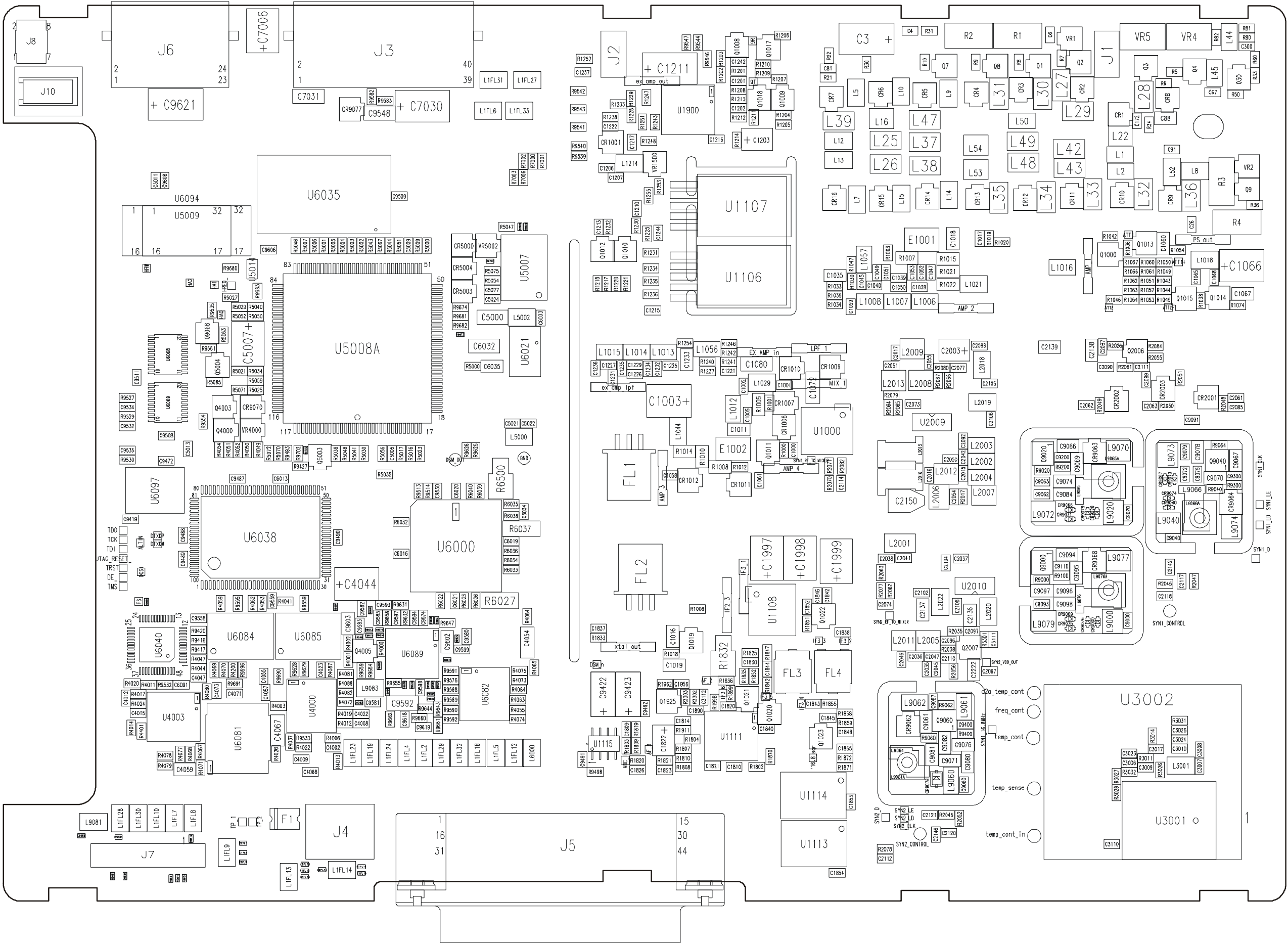
Figure B-3.A. LORD Module, Identification of Components (Sheet 1 of 2)
