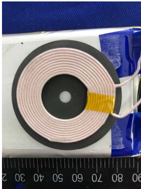
EUT – Coil View
