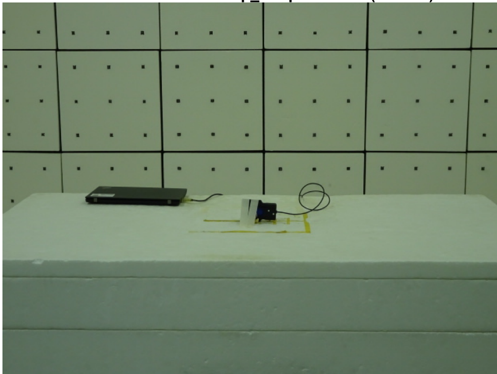
Front View of test setup_Loop Antenna (C-Intac)
