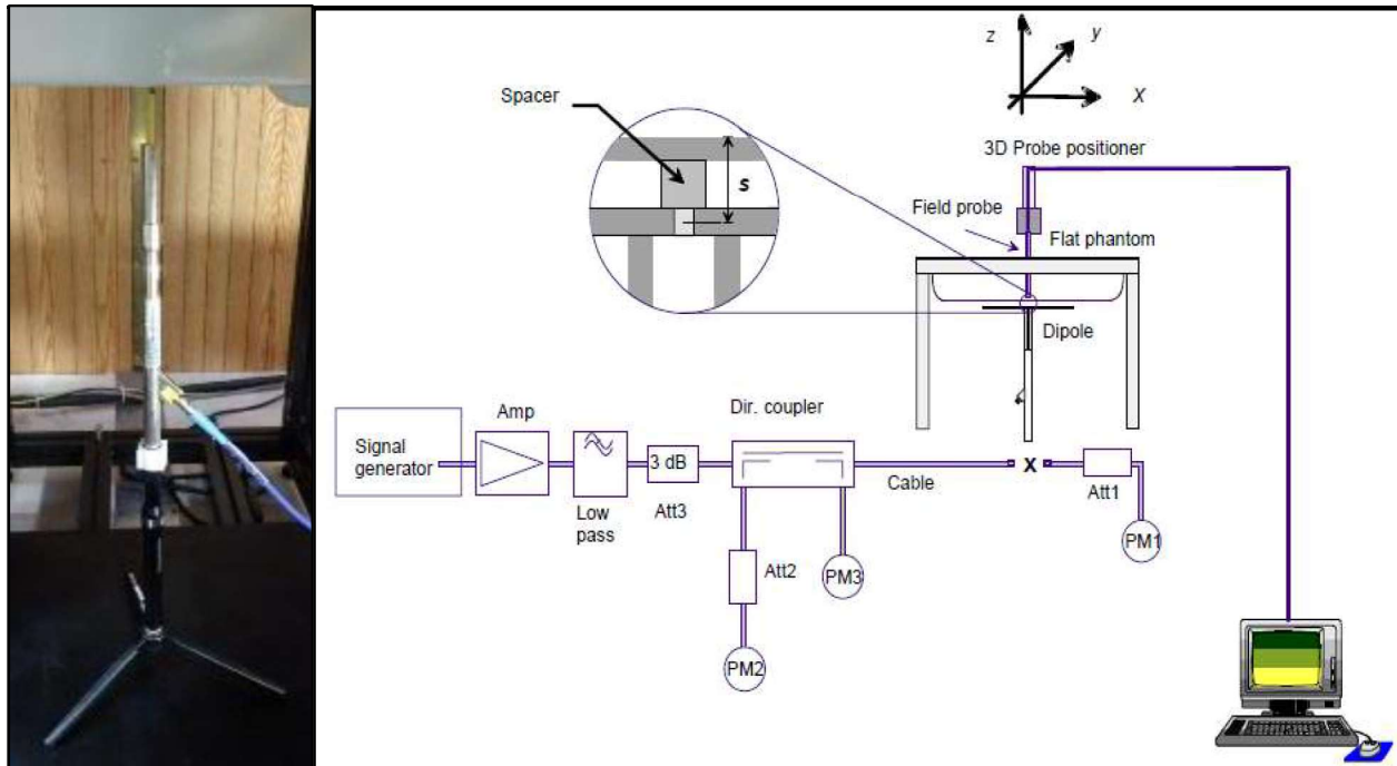
Figure 11: System Verification Setup
