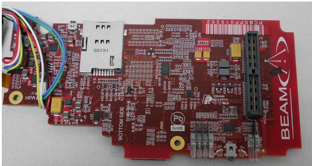
PCB Top and Bottom
