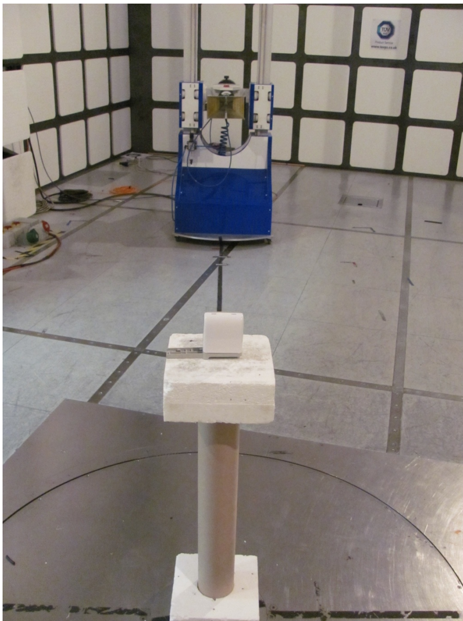
Radiated Emissions 1GHz to 10GHz
