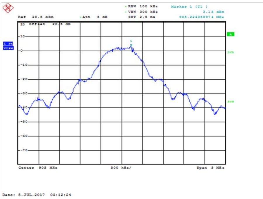
Figure 3 - 905 MHz
