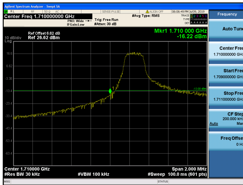
Band4-1.4MHz-QPSK-19957-6RB#0
