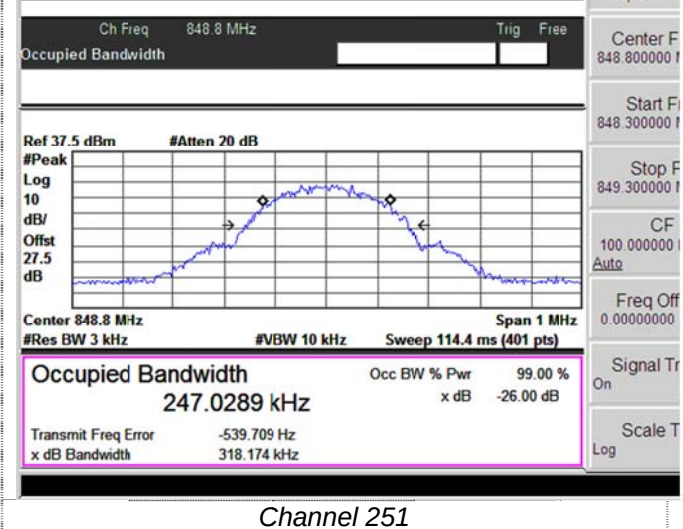
99% Occupy bandwidth&-26dB bandwidth
