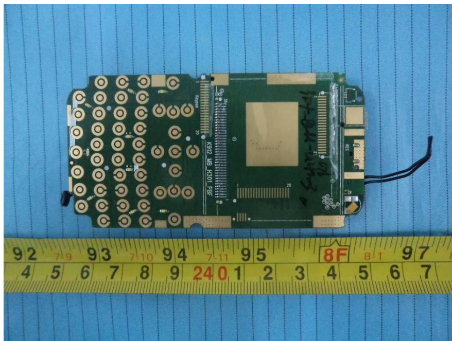
EUT – Main Board Bottom without Keypad View
