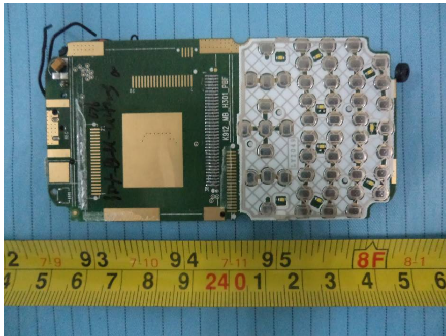
EUT – Main Board Bottom with Keypad View
