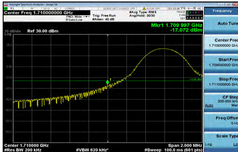
Band4-10MHz-QPSK-20000-1RB#49
