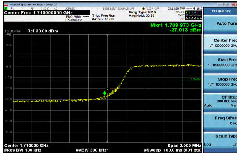
Band4-5MHz-QPSK-20375-1RB#24
