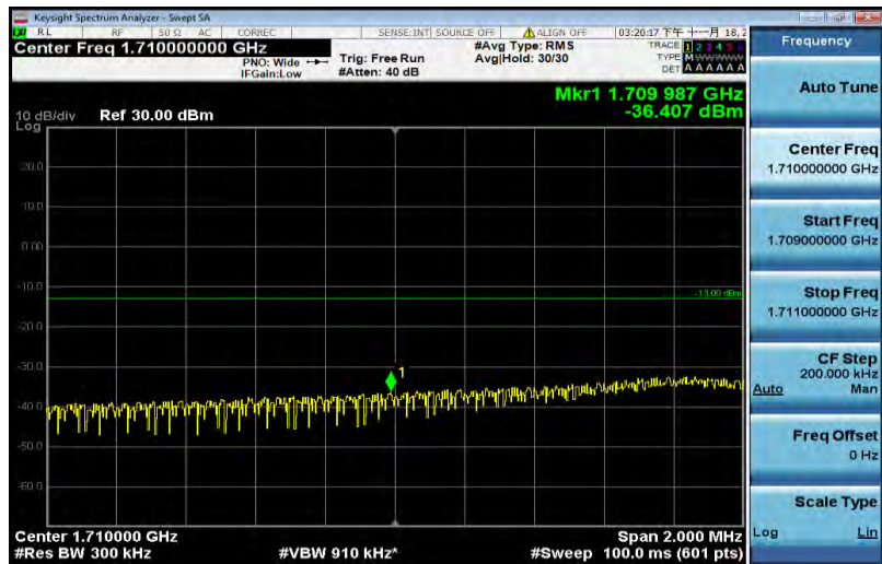
Band4-15MHz-16QAM-20025-75RB#0
