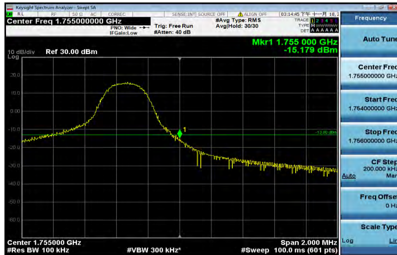
Band4-5MHz-QPSK-20375-1RB#0
