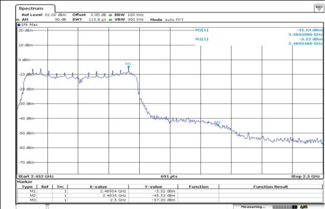
CH11-Bandedge
