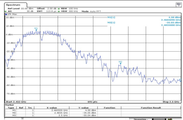
CH11-Bandedge
