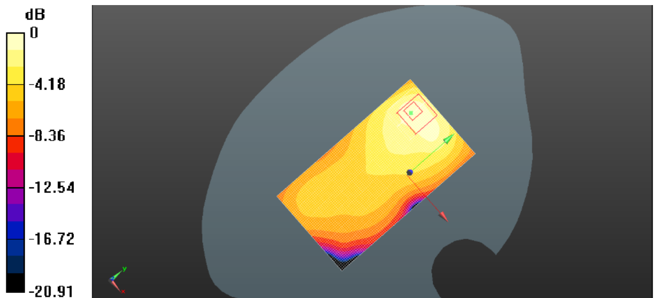
Plot 8: Body Rear Side (WCDMA Band II RMC Middle Channel)
