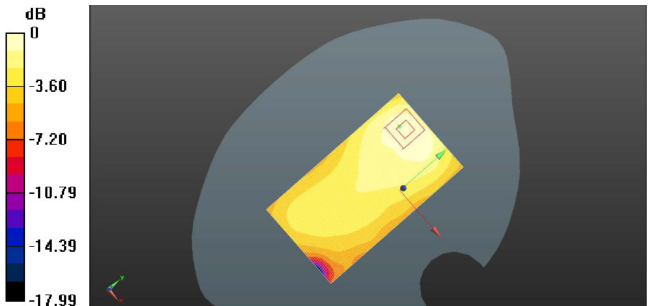
Plot 4: Body Rear Side (GSM1900 EGPRS 2TS Middle Channel)
