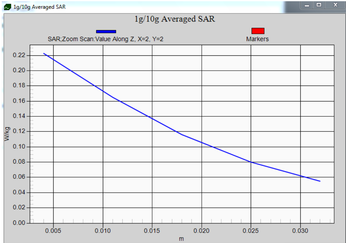
Z-Scan at power reference point- Left Head Tilt (WCDMA Band II Middle Channel)
