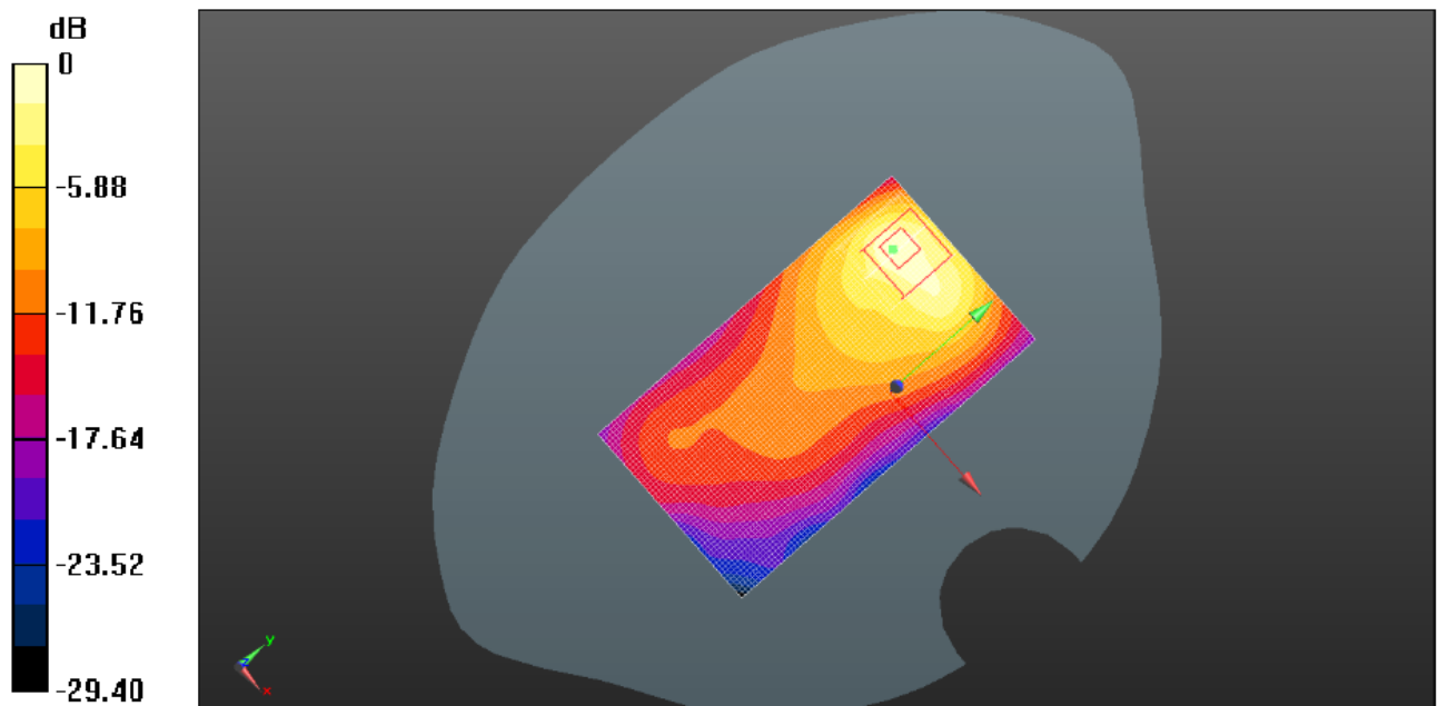
Plot 6: Body Rear Side (WCDMA Band V RMC Middle Channel)
