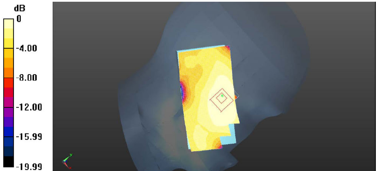
Plot 1: Left Head Tilt (GSM850 Middle Channel)
