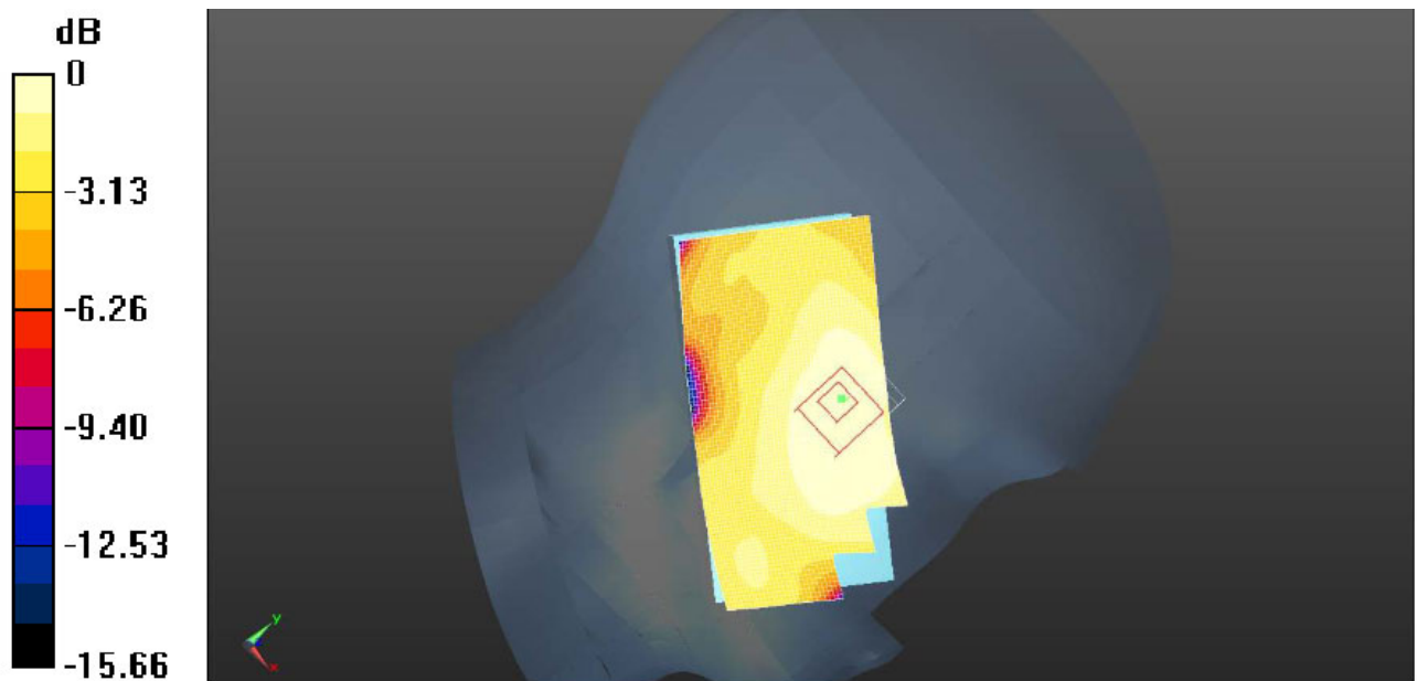
Plot 9: Left Head Tilt (WLAN2450 Middle Channel-Channel 6-2437MHz (1Mbps))
