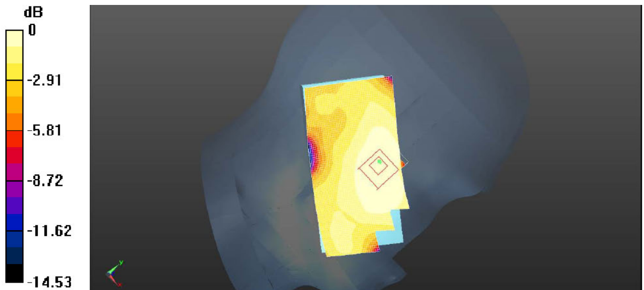
Plot 3: Left Head Touch (GSM1900 Middle Channel)
