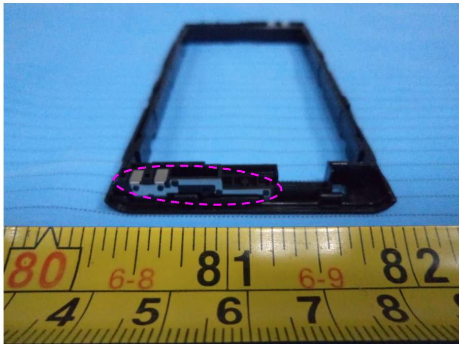
EUT – LTE(MIMO) Antenna View
