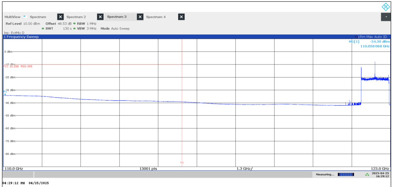
Plot 46: 110 GHz – 123 GHz, normal operation mode (in-band wanted signal visible on plot)
