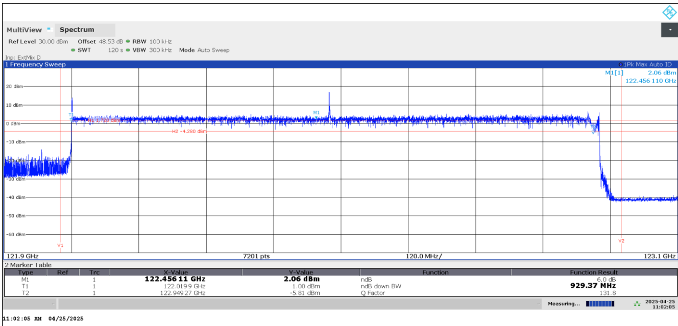
Plot 2: EUT 1, Normal Mode, 6 dB bandwidth (RBW = 100 kHz)
