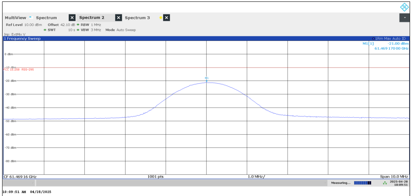
Plot 36: 50 GHz – 75 GHz, stop mode, high frequency, 10 MHz span
