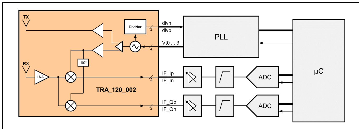
Figure 6 Application Circuit
