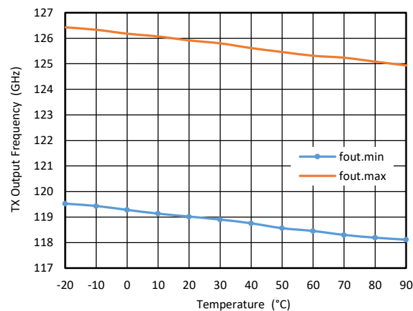
Figure 15 Output Frequency vs. Temperature
