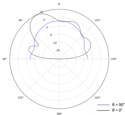
Figure 18 Antenna Radiation Pattern (simulated)
