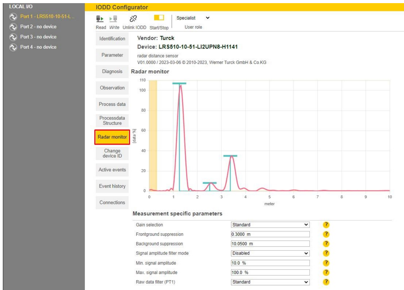
Fig. 21: Turck Radar Monitor – overview
