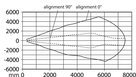
Fig. 10: DR...WE... range diagram
