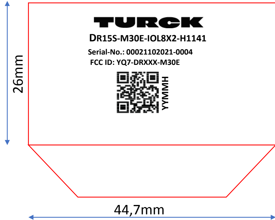
Device marking
