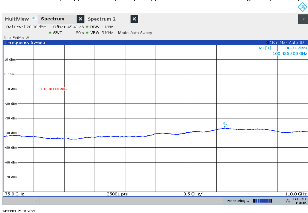
Plot 29: 75 GHz – 110 GHz, stopped mode (sweep stopped in the middle of the range of operation)
