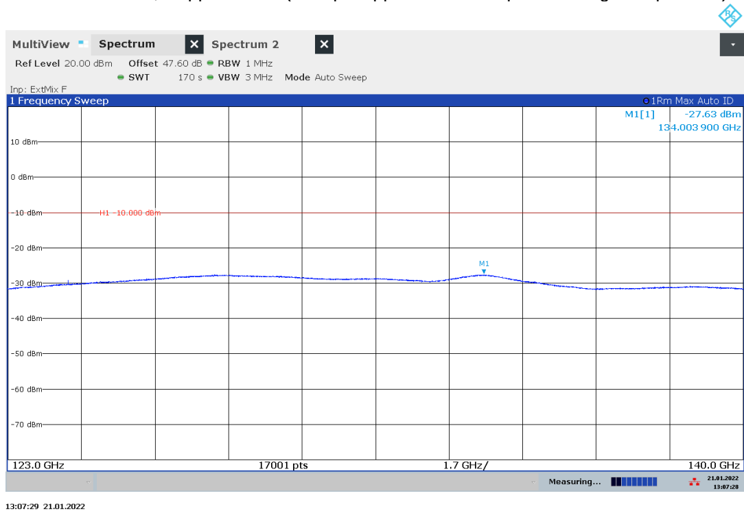
Plot 33: 123 GHz – 140 GHz, stopped mode (sweep stopped near the top of the range of operation)
