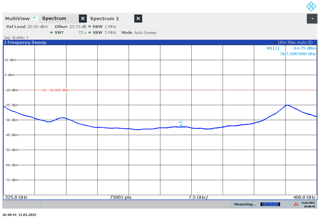
Plot 42: 325 GHz – 400 GHz, normal mode
