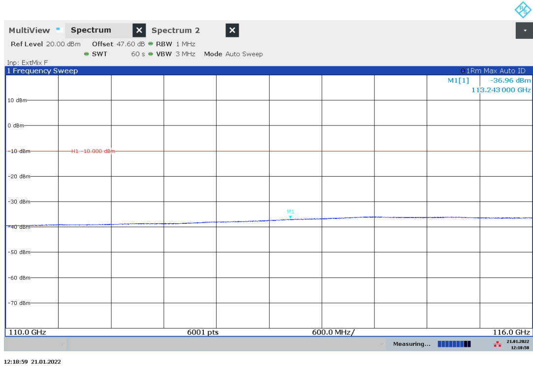
Plot 30: 110 GHz – 116 GHz, normal mode
