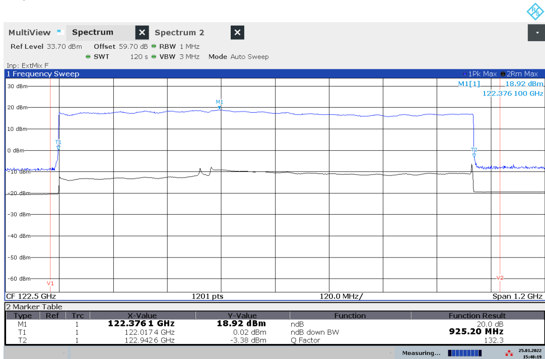
Plot 47: Occupied Bandwidth at 20 °C / V max
