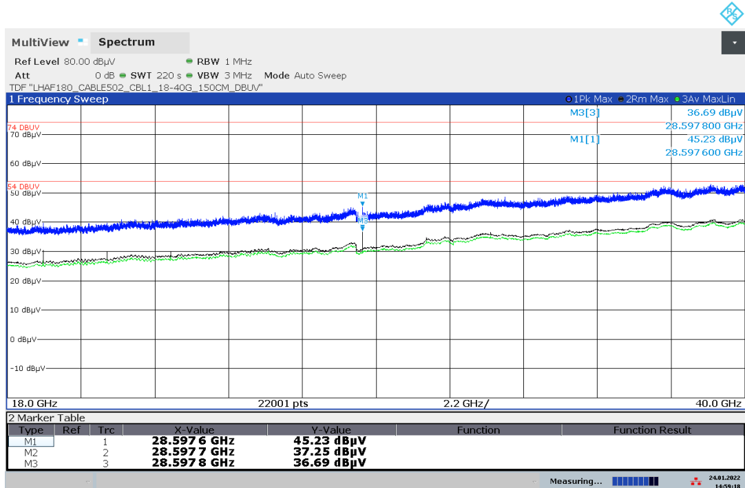
Plot 16: 18 GHz – 40 GHz, stopped mode (sweep stopped near the bottom edge of the range of operation)
