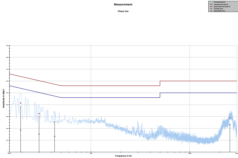
Plot 49: Phase line
