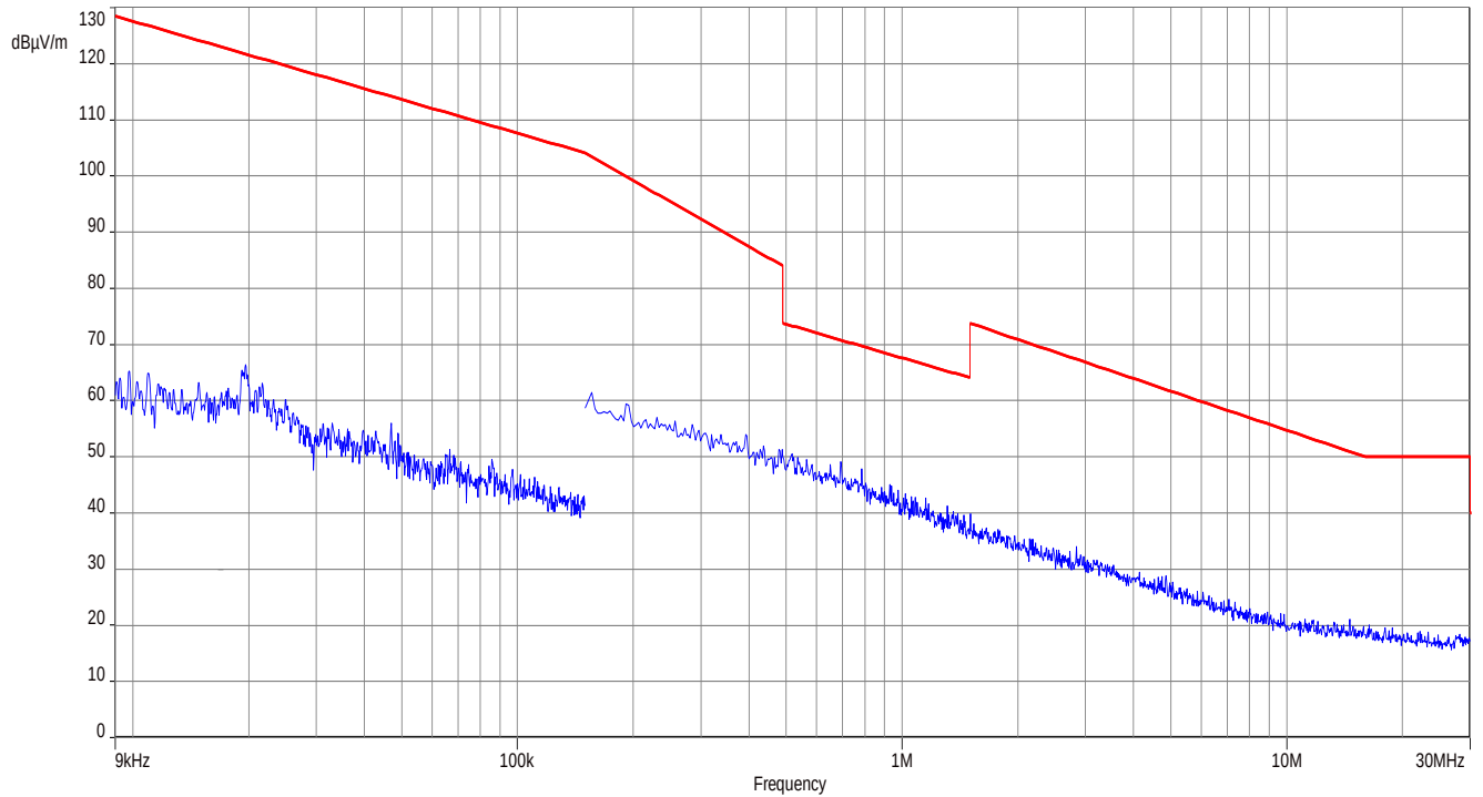
Plot 5: 9 kHz – 30 MHz, normal mode
