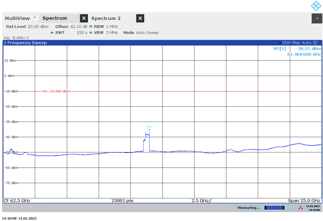
Plot 20: 50 GHz – 75 GHz, normal mode
