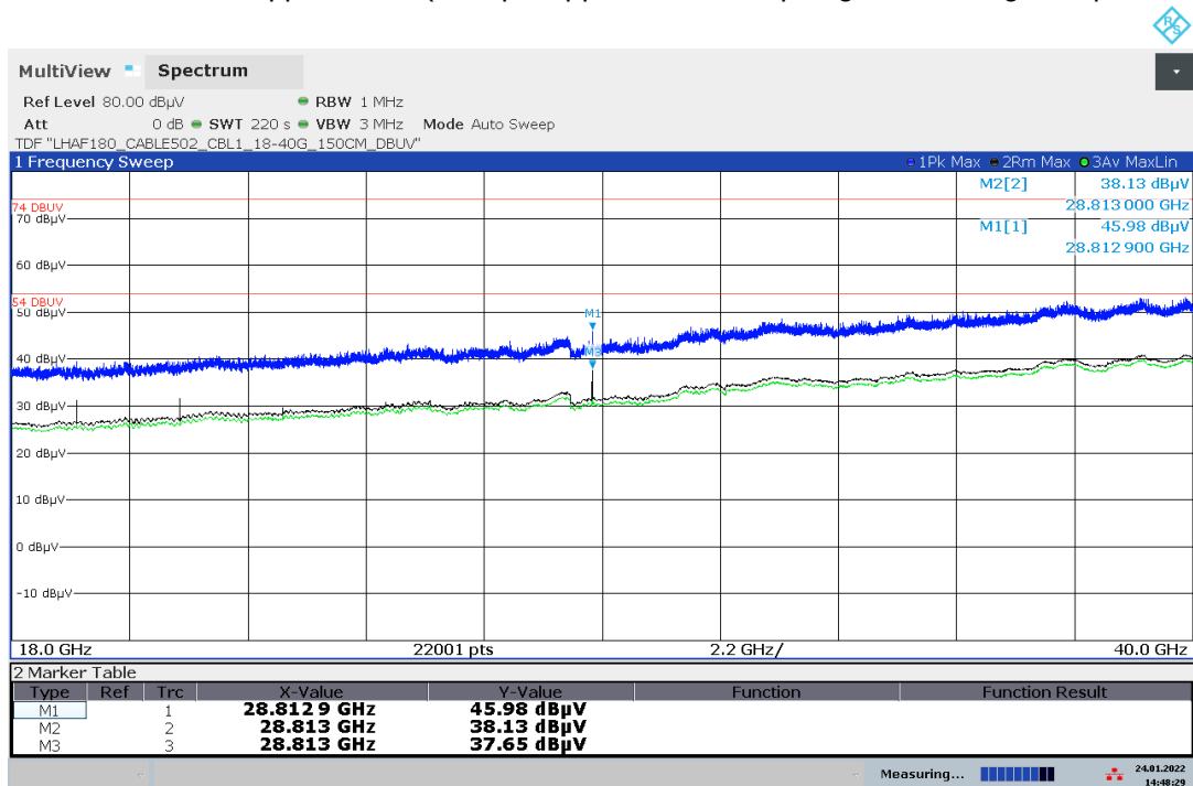
Plot 17: 18 GHz – 40 GHz, stopped mode (sweep stopped near the top edge of the range of operation)
