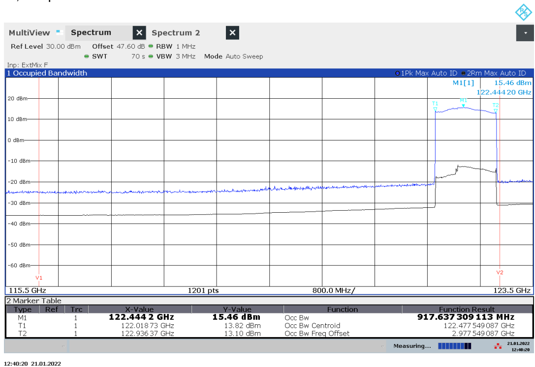
Plot 4: OBW, complete band
