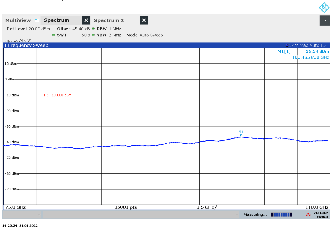
Plot 28: 75 GHz –110 GHz, normal mode
