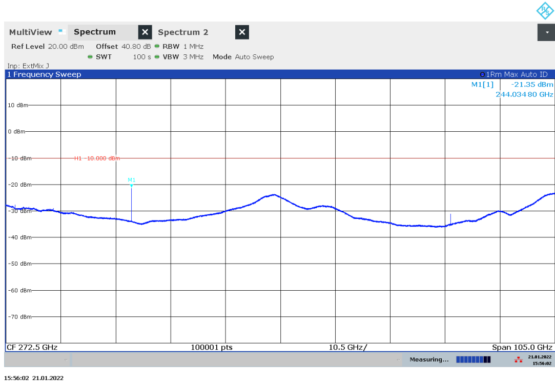
Plot 39: 220 GHz – 325 GHz, stopped mode (sweep stopped near the bottom of the range of operation)
