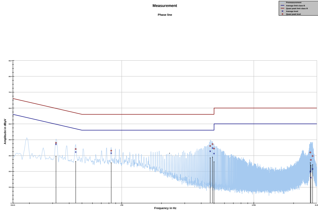
Plot 77: Phase line 1" version
