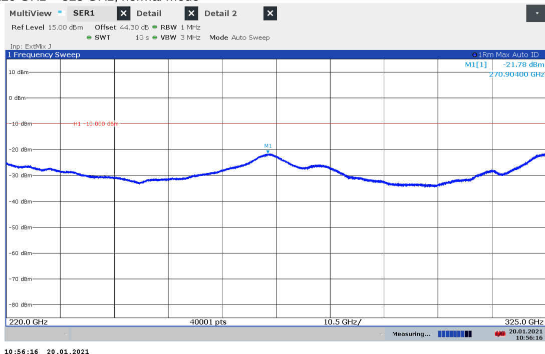
Plot 65: 220 GHz – 325 GHz, normal mode
