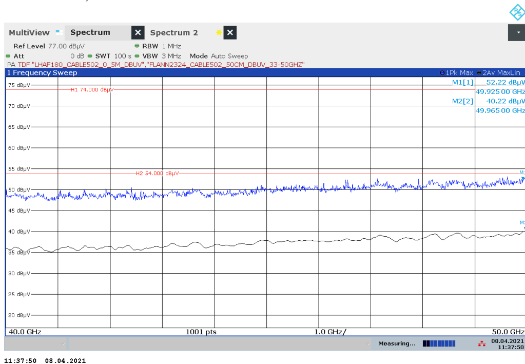
Plot 15: 40 GHz – 50 GHz, normal mode
