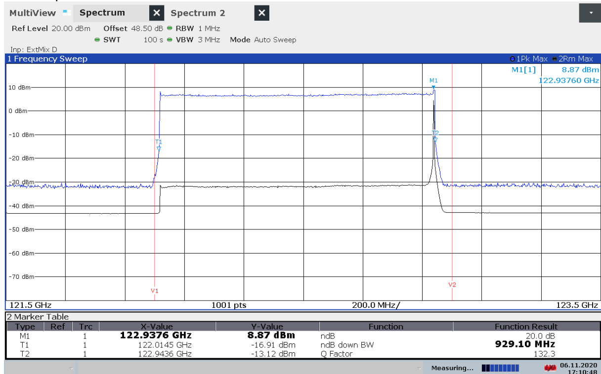
Plot 69: Occupied Bandwidth of 1" version at -20 °C / V nom
