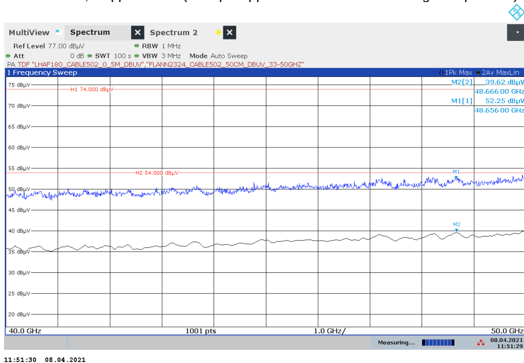
Plot 16: 40 GHz – 50 GHz, stopped mode (sweep stopped in the middle of the range of operation)
