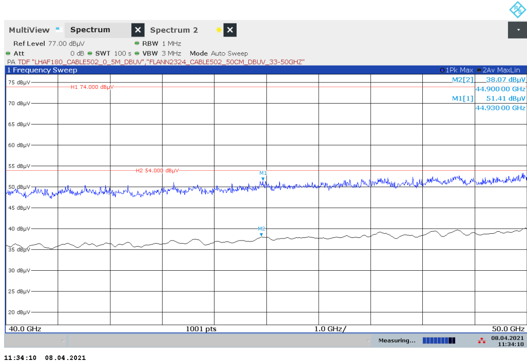
Plot 47: 40 GHz – 50 GHz, normal mode
