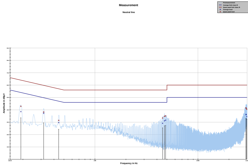
Plot 80: Neutral line ¾" version
