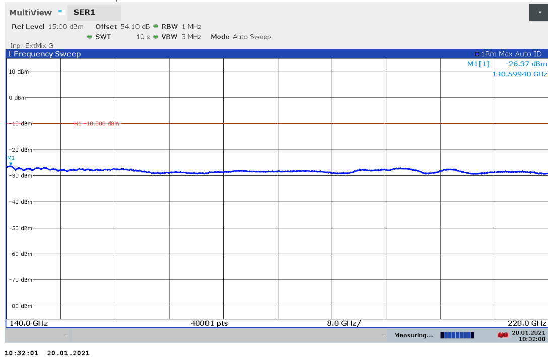
Plot 31: 140 GHz – 220 GHz, normal mode
