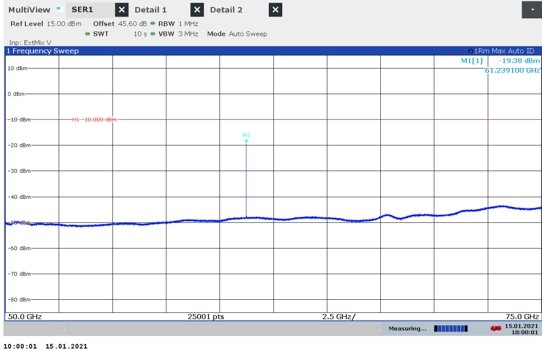
Plot 53: 50 GHz – 75 GHz, stopped mode (sweep stopped in the middle of the range of operation)
