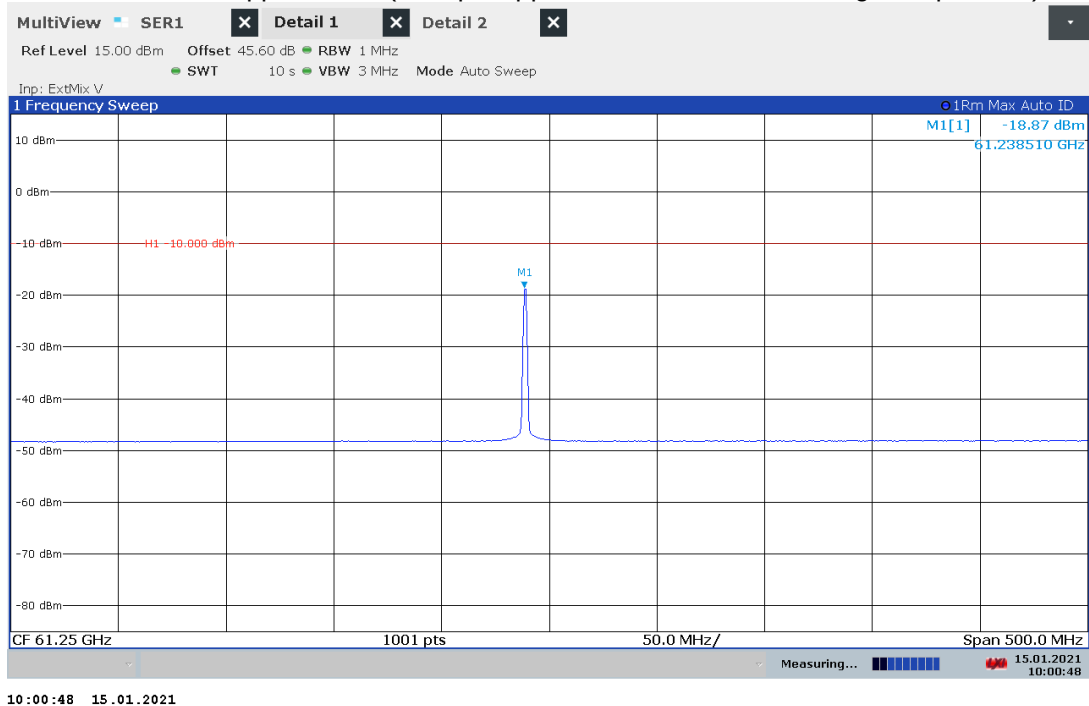
Plot 54: 50 GHz – 75 GHz, stopped mode (sweep stopped in the middle of the range of operation)
