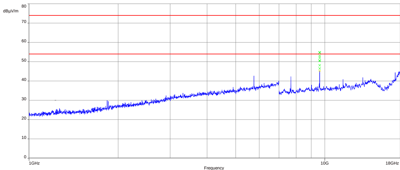
Plot 9: 1 GHz – 18 GHz, normal mode
