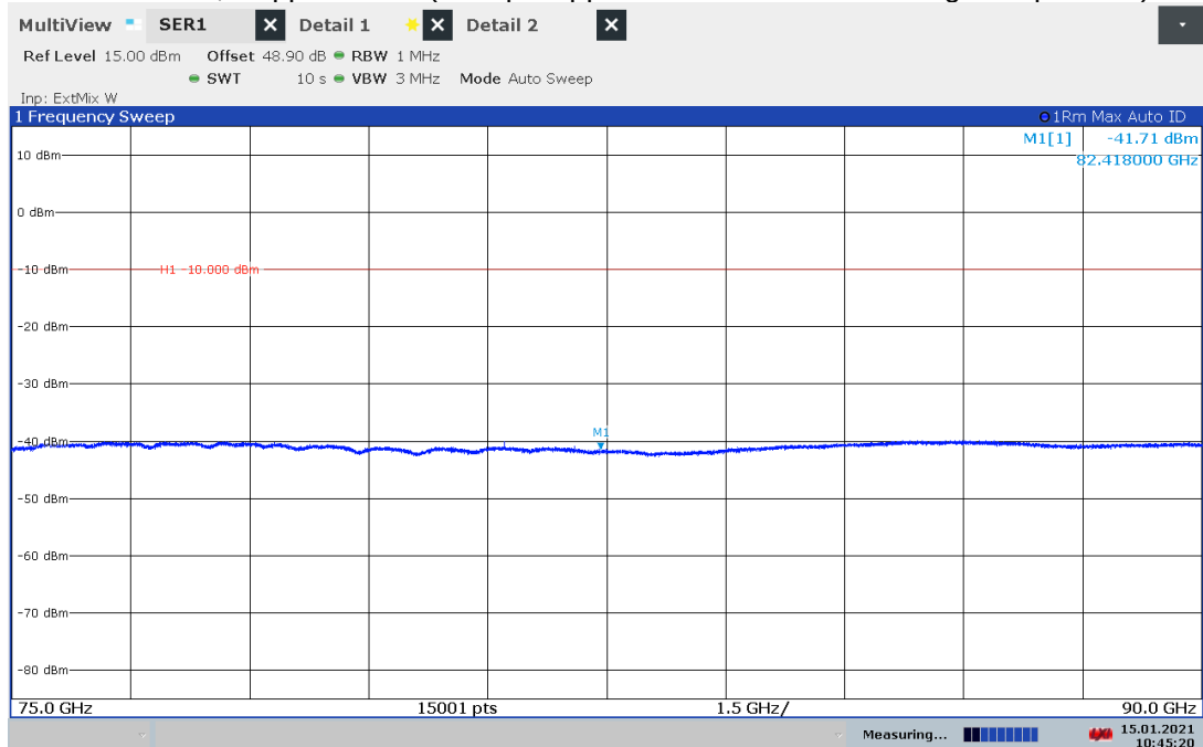
Plot 26: 75 GHz – 90 GHz, stopped mode (sweep stopped in the middle of the range of operation)
