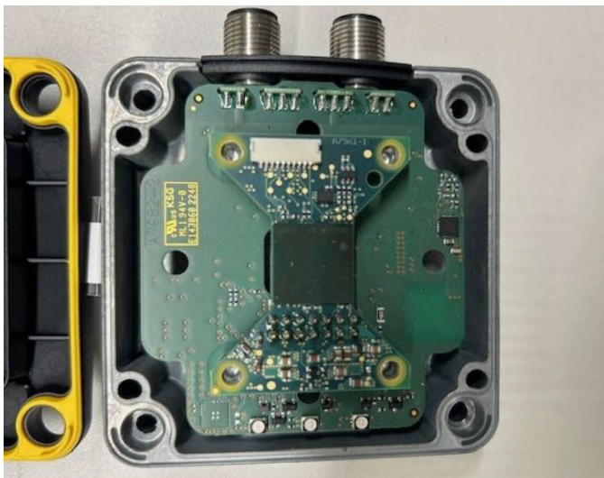
Photo 2: Inside View 2
