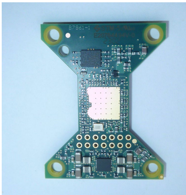
Photo 4: B7961-1
