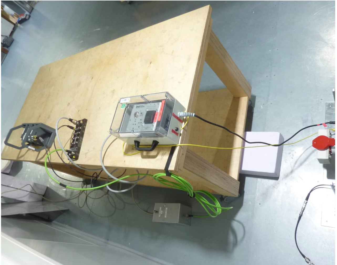
Setup power-line conducted: 150kHz – 30 MHz
