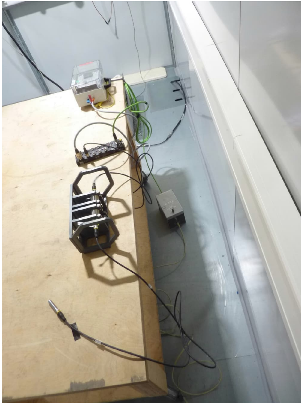
Setup power-line conducted: 150kHz – 30 MHz
