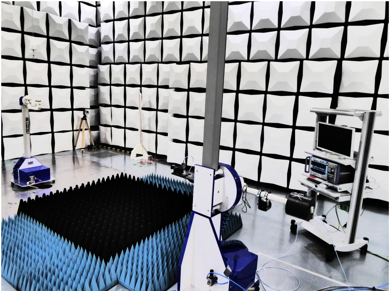
Test setup semi anechoic chamber with ground plane (18 – 26.5 GHz)
