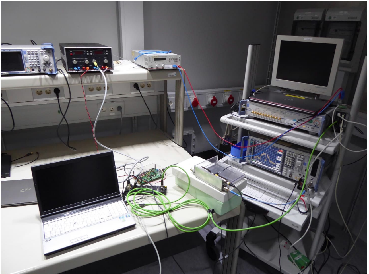
Test setup antenna port conducted – measurement with coupling plate
