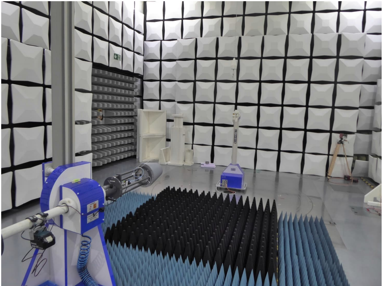
Test setup semi anechoic chamber with ground plane (1 - 18 GHz)
