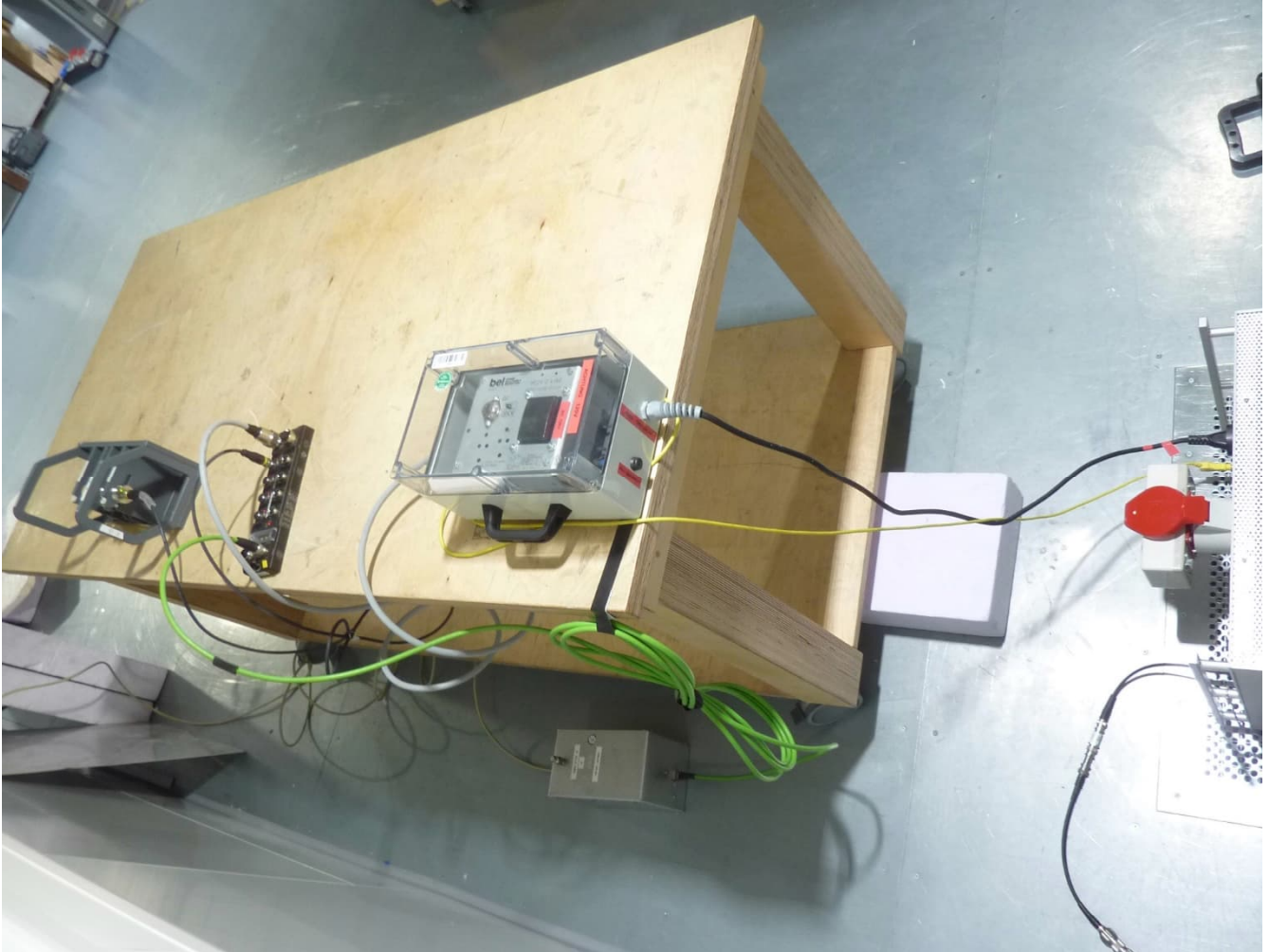
Setup power-line conducted: 150kHz – 30 MHz
