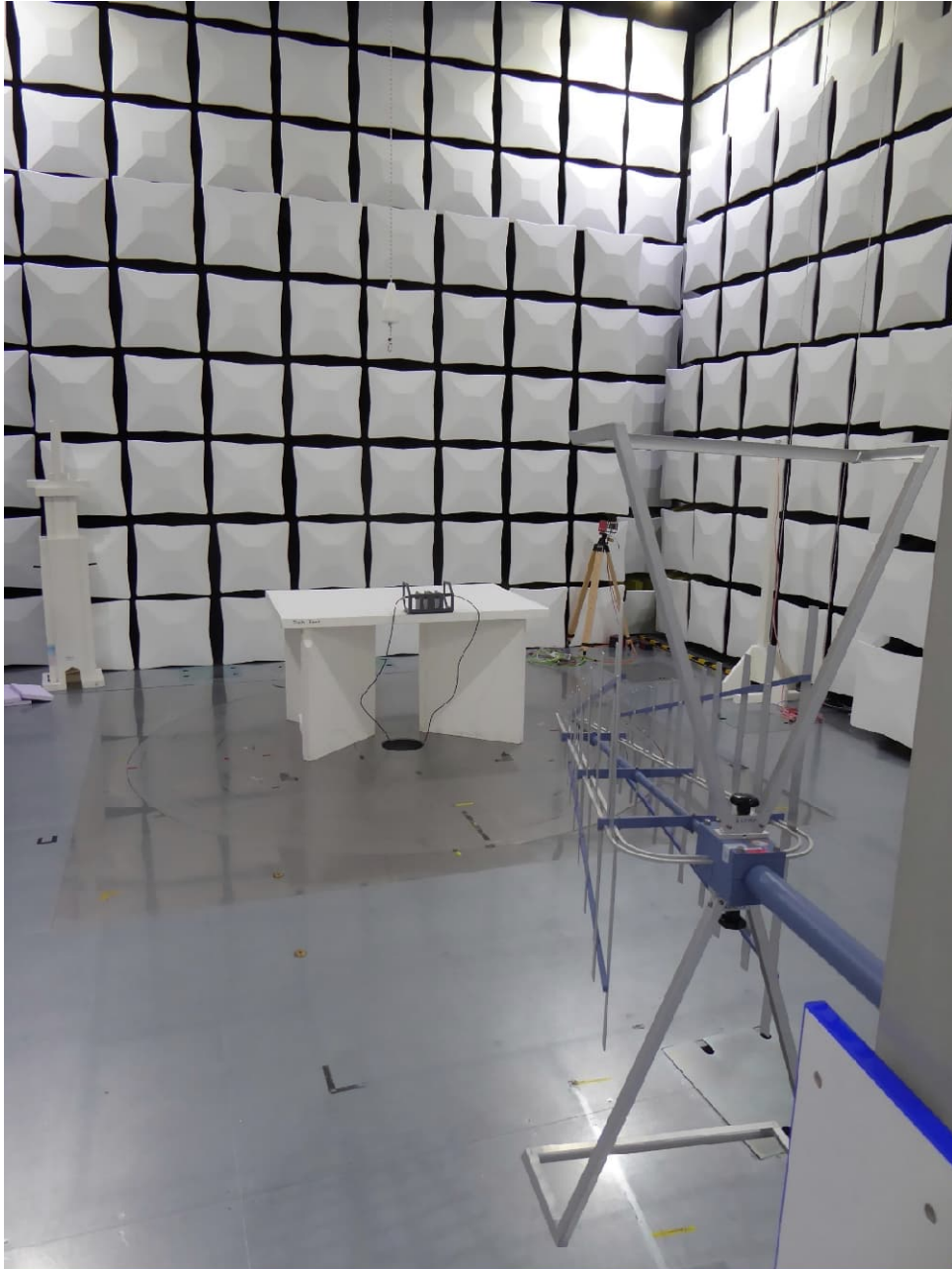
Setup Radiated: 30 MHz - 1 GHz
