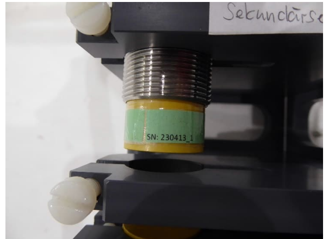
Setup Radiated
