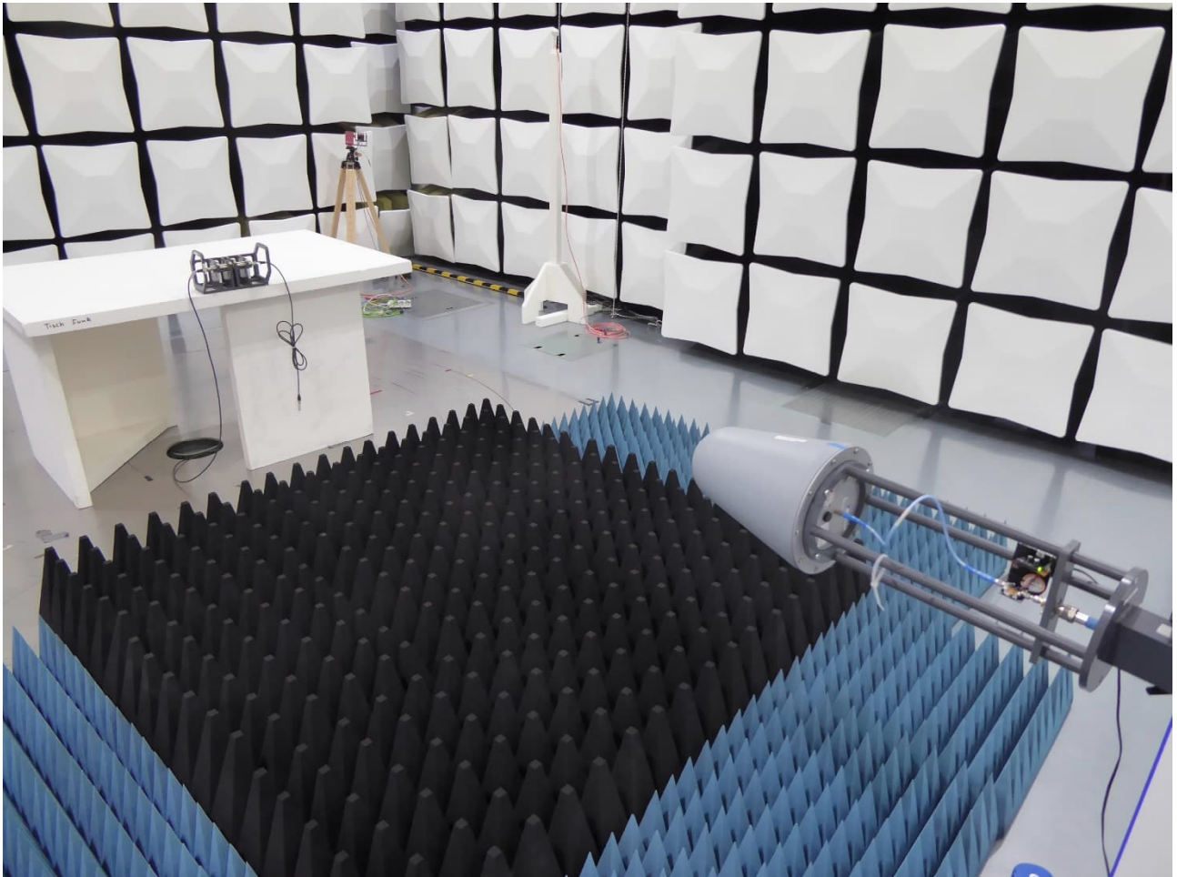
Setup Radiated: 1 GHz - 12 GHz
