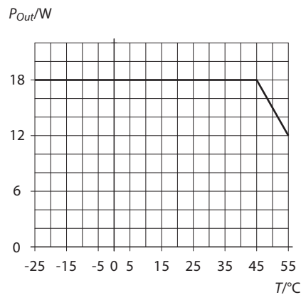
Fig. 11: Temperature derating
