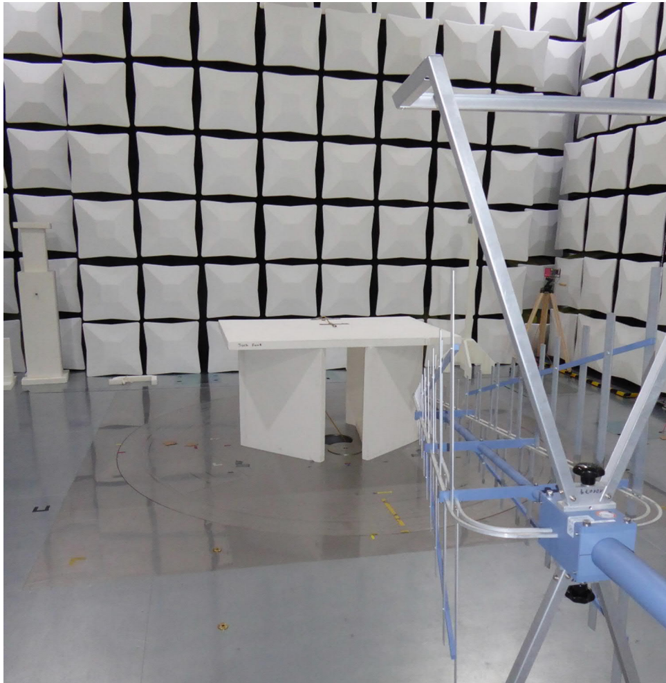
Test setup semi anechoic chamber (30 MHz to 1 GHz)
