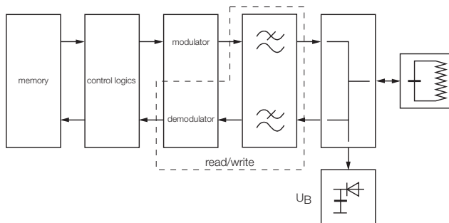
Figure 1 Block diagram Data carrier
