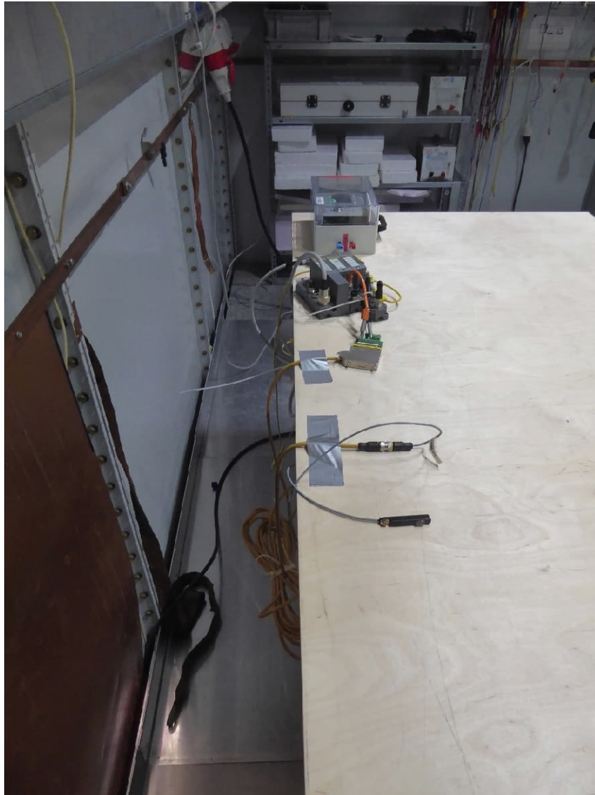
AC Mains conducted emissions test setup
