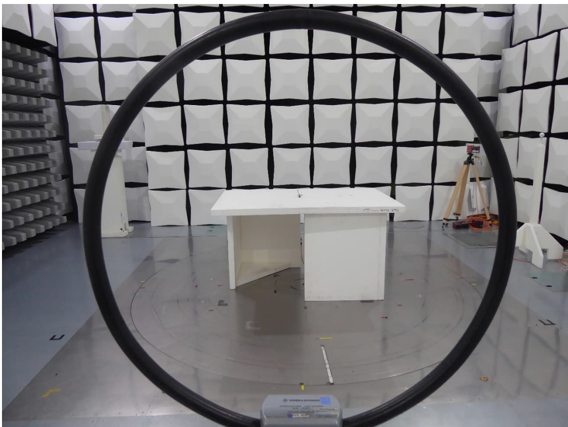
Test setup semi anechoic chamber (9 kHz to 30 MHz)
