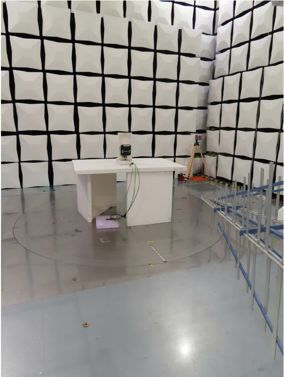
30 MHz – 1 GHz - EUT position 1
