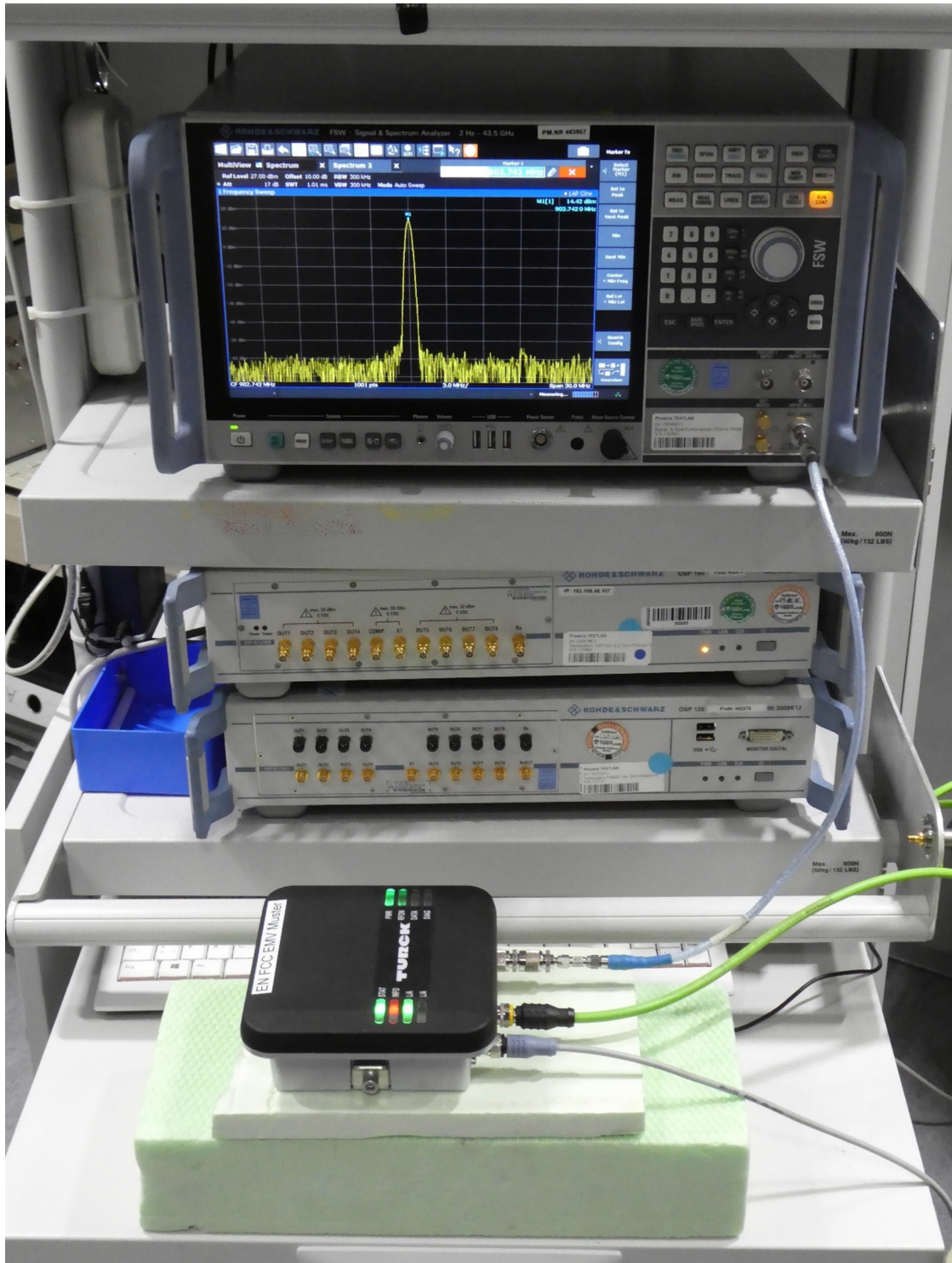
Test setup - conducted @ antenna port
