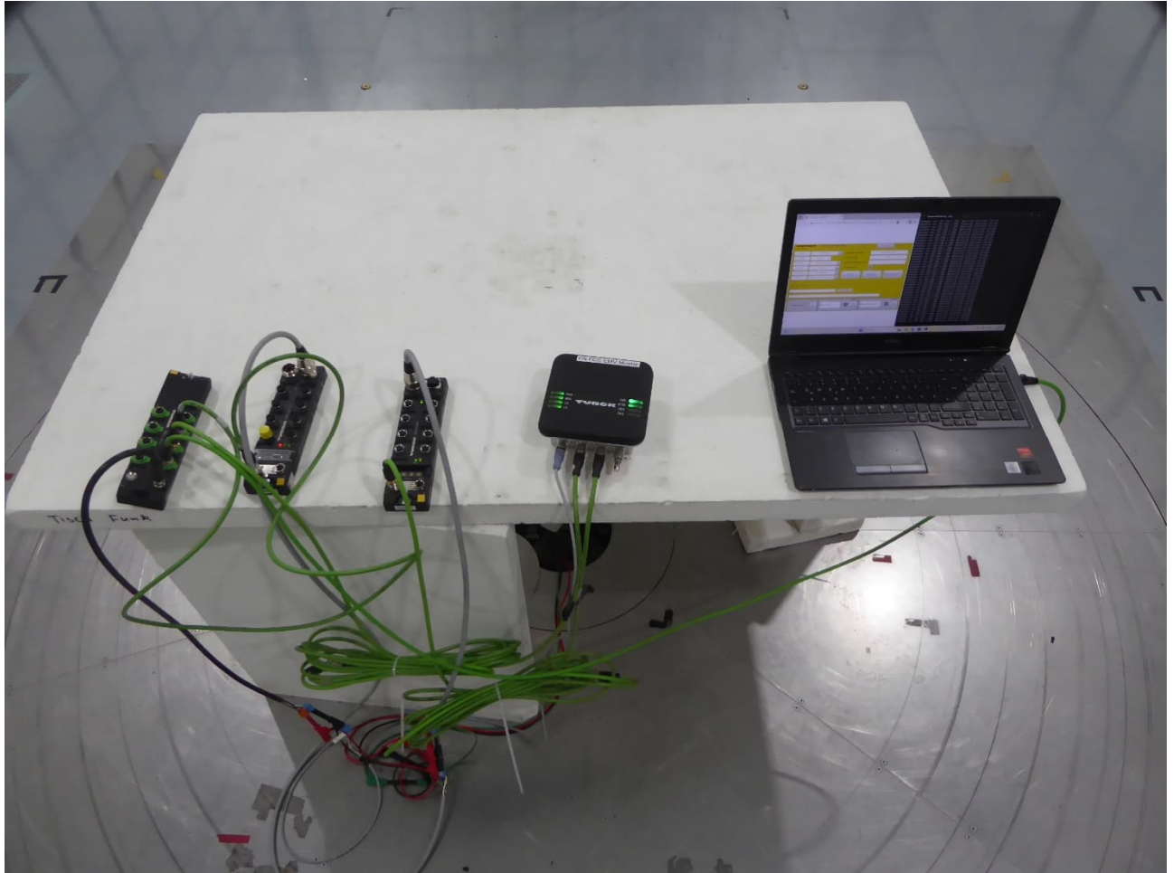
Radiated emissions - EUT position 2
