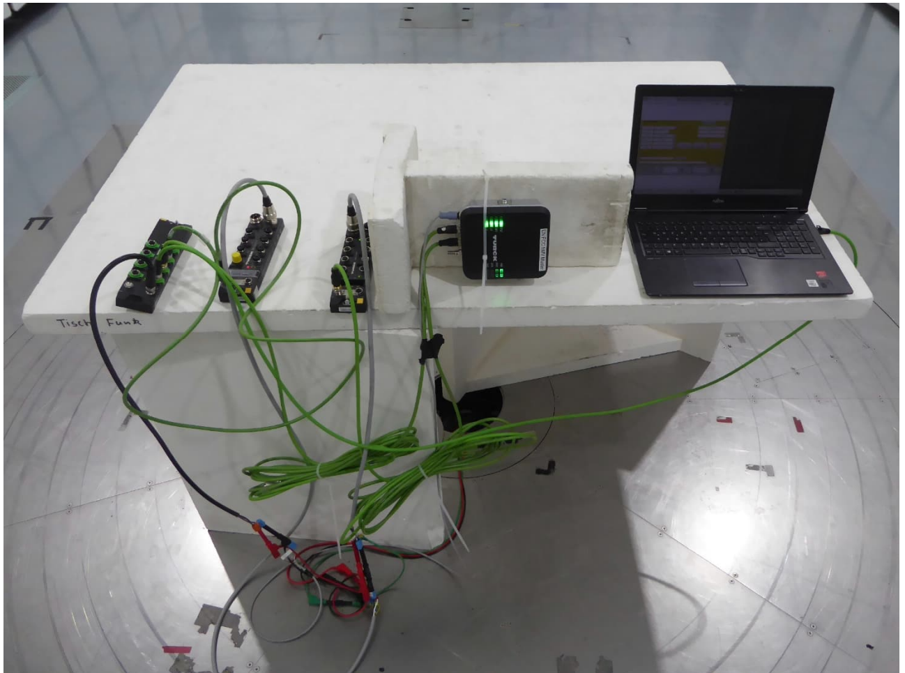
Radiated emissions - EUT position 3
