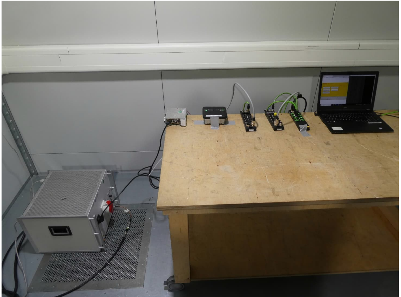
AC power line conducted emissions - EUT 1
