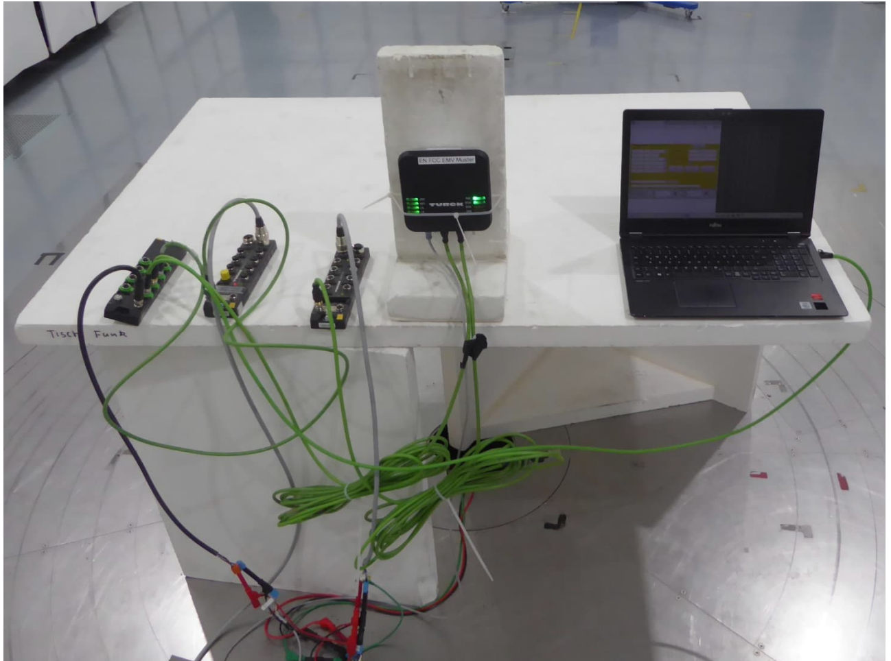
Radiated emissions - EUT position 1
