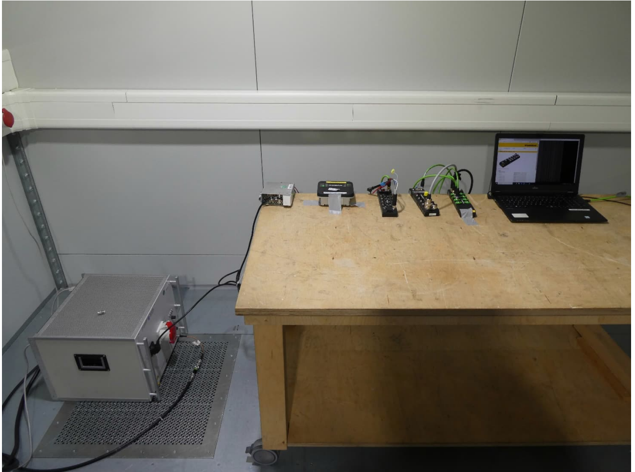
AC power line conducted emissions - EUT 2
