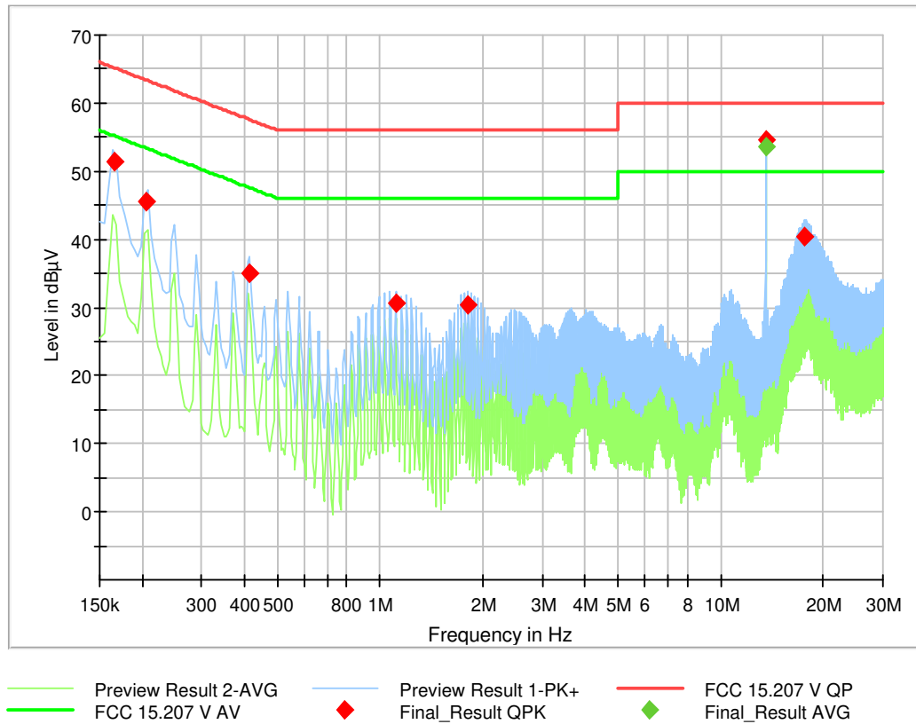
Test plot for AC mains conducted emissions with antenna
