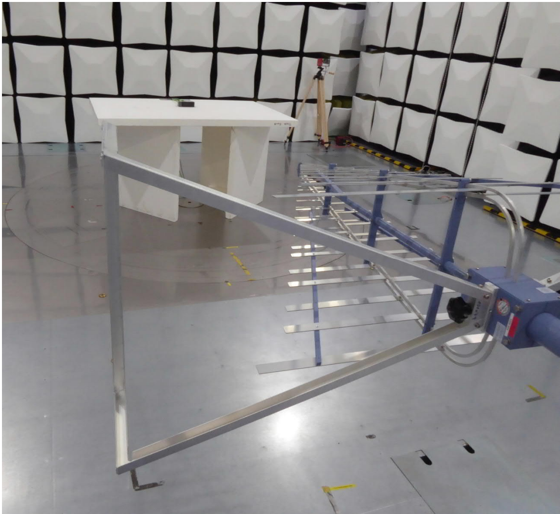
Test setup semi anechoic chamber (30 MHz to 1 GHz)
