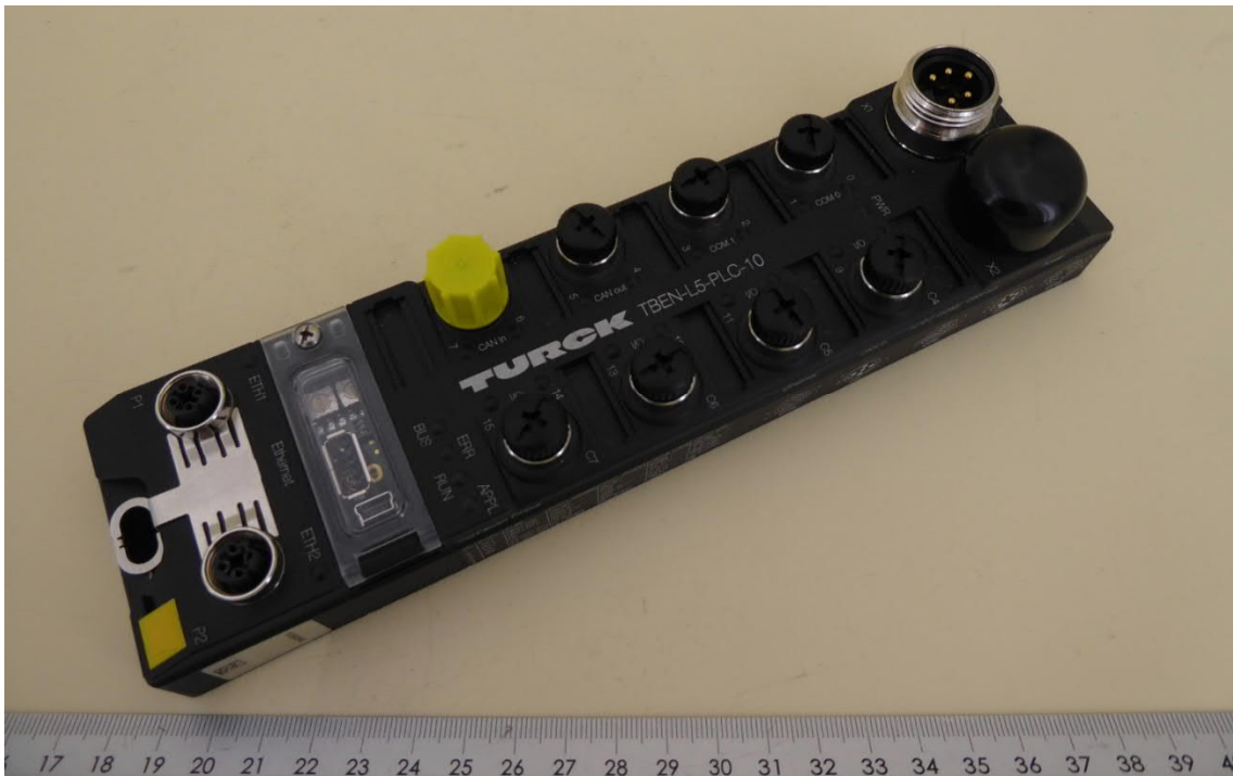
TURCK Gateway TBEN-L5-PLC-10
